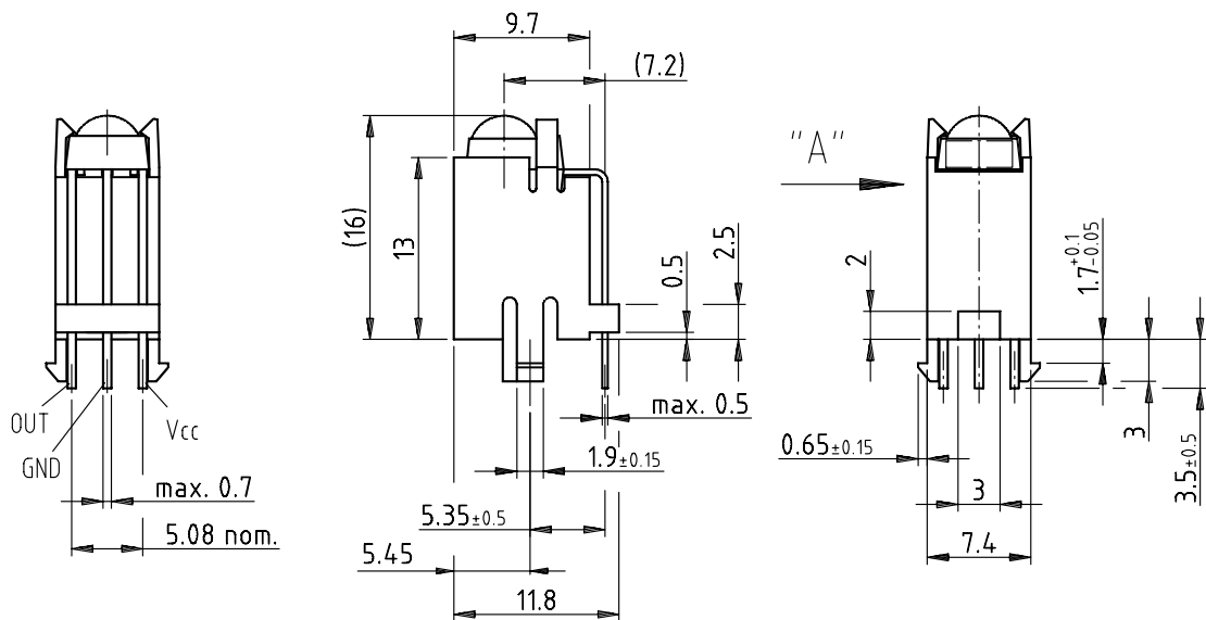
View "A"
