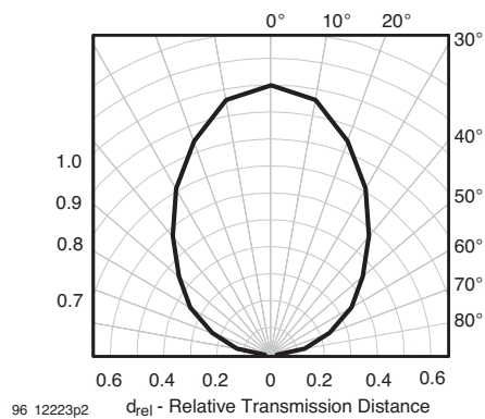
Figure 12. Directivity
