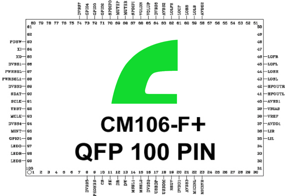
Figure 1. CM106-F+ QFP 100 Pin Assignments (Top View)
