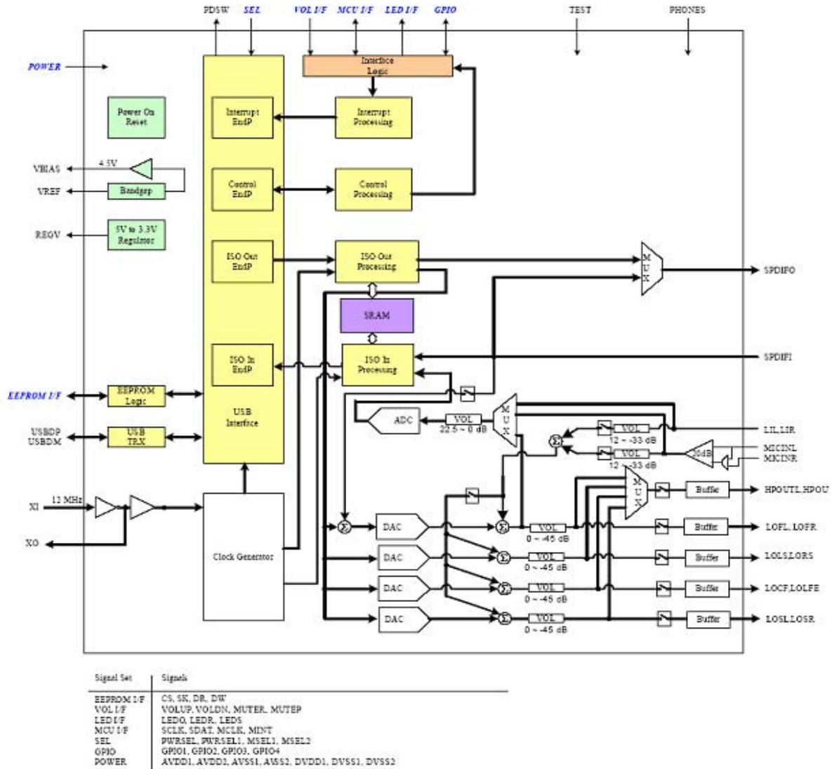
Figure 3 : Function Block Diagram Of CM106-F+/L+
