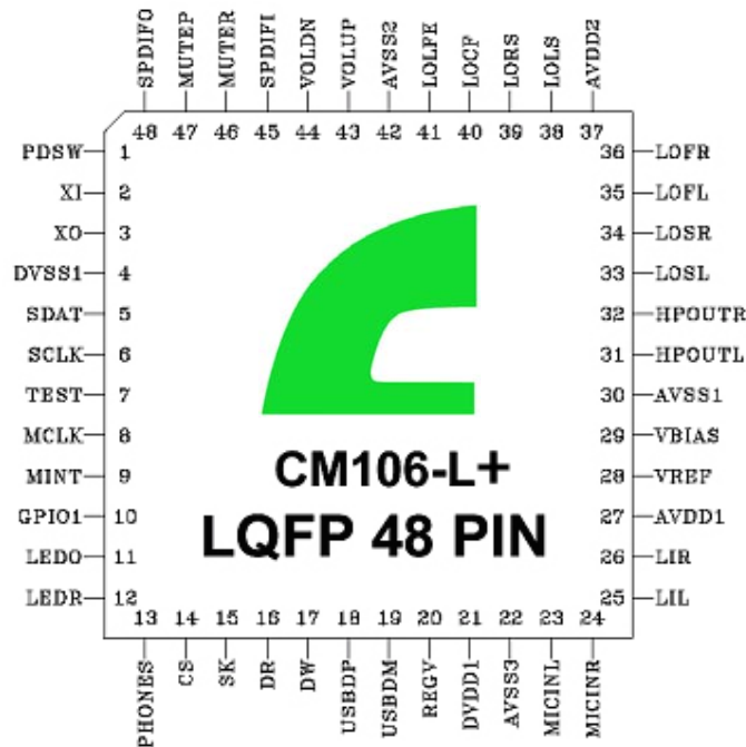
Figure 2. CM106-L+ LQFP 48 Pin Assignments (Top View)
