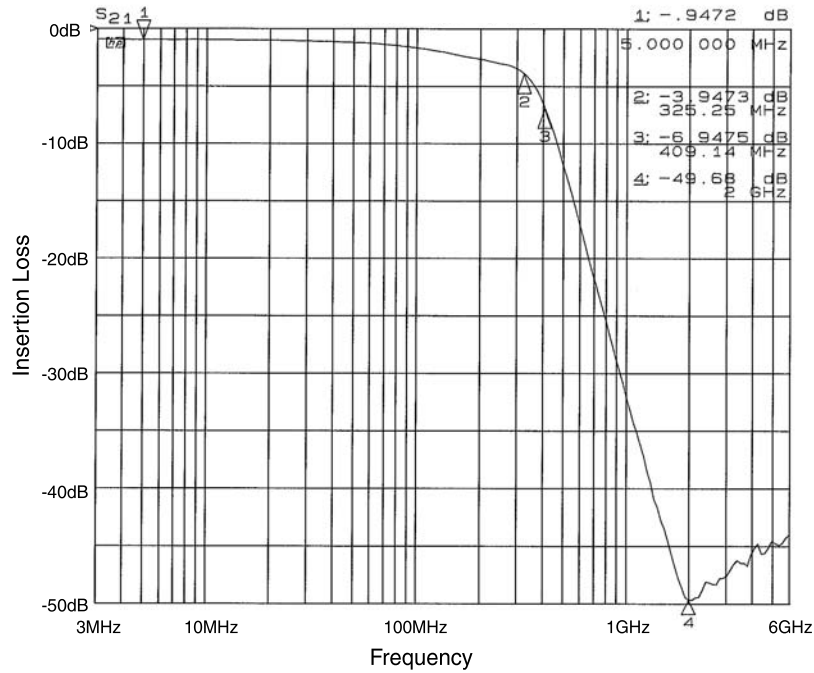
Figure 5. Filter 5 Insertion Loss (CM1661-06DE)
