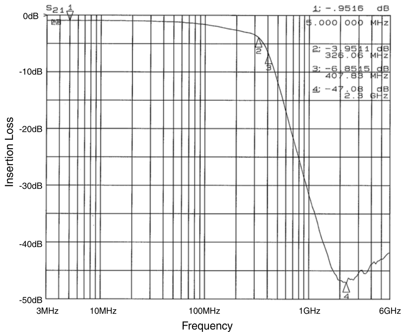
Figure 4. Filter 4 Insertion Loss (CM1661-06DE)
