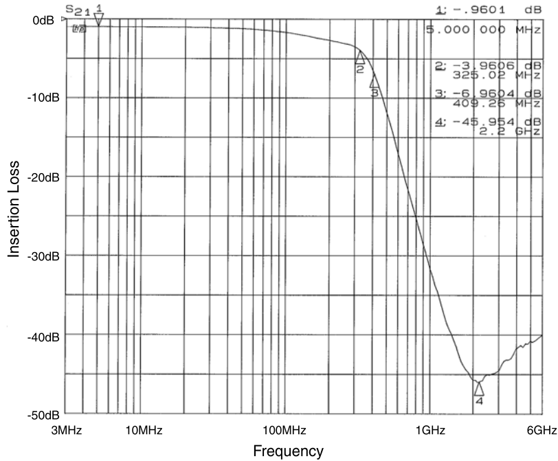
Figure 3. Filter 3 Insertion Loss (CM1661-06DE)
