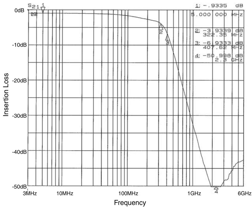
Figure 6. Filter 6 Insertion Loss (CM1661-06DE)
