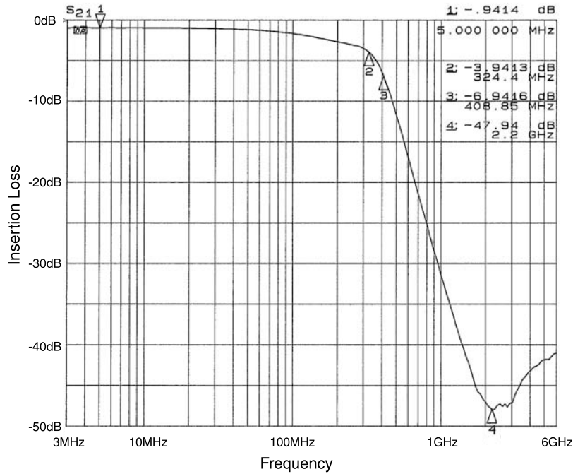
Figure 1. Filter 1 Insertion Loss (CM1661-06DE)
