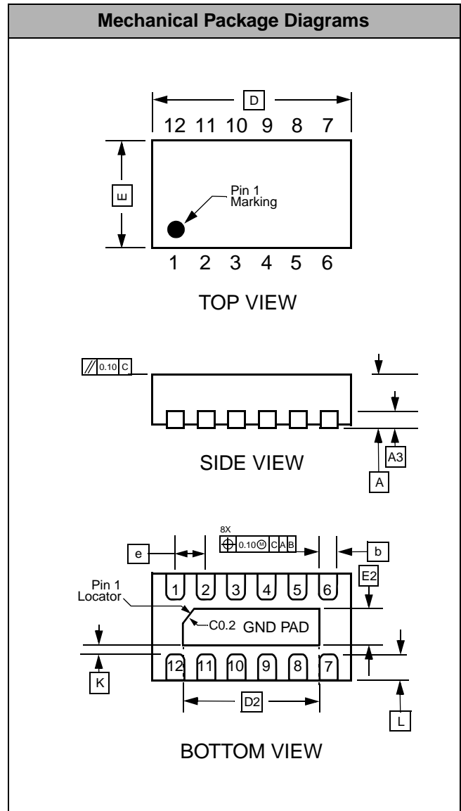
Dimensions for 12-Lead, 3.00mm x 1.35mm, 0.5mm pitch uDFN package
