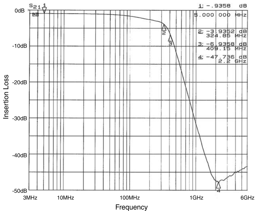
Figure 2. Filter 2 Insertion Loss (CM1661-06DE)
