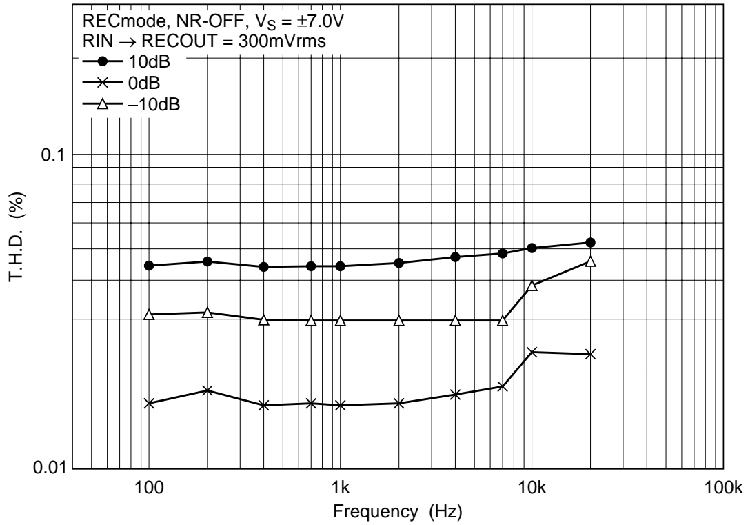
Total Harmonic Distortion vs. Frequency (1)
