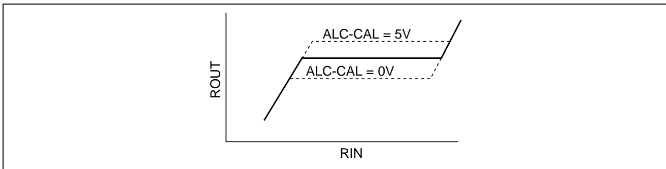
Figure 13 ALC-CAL Characteristics
