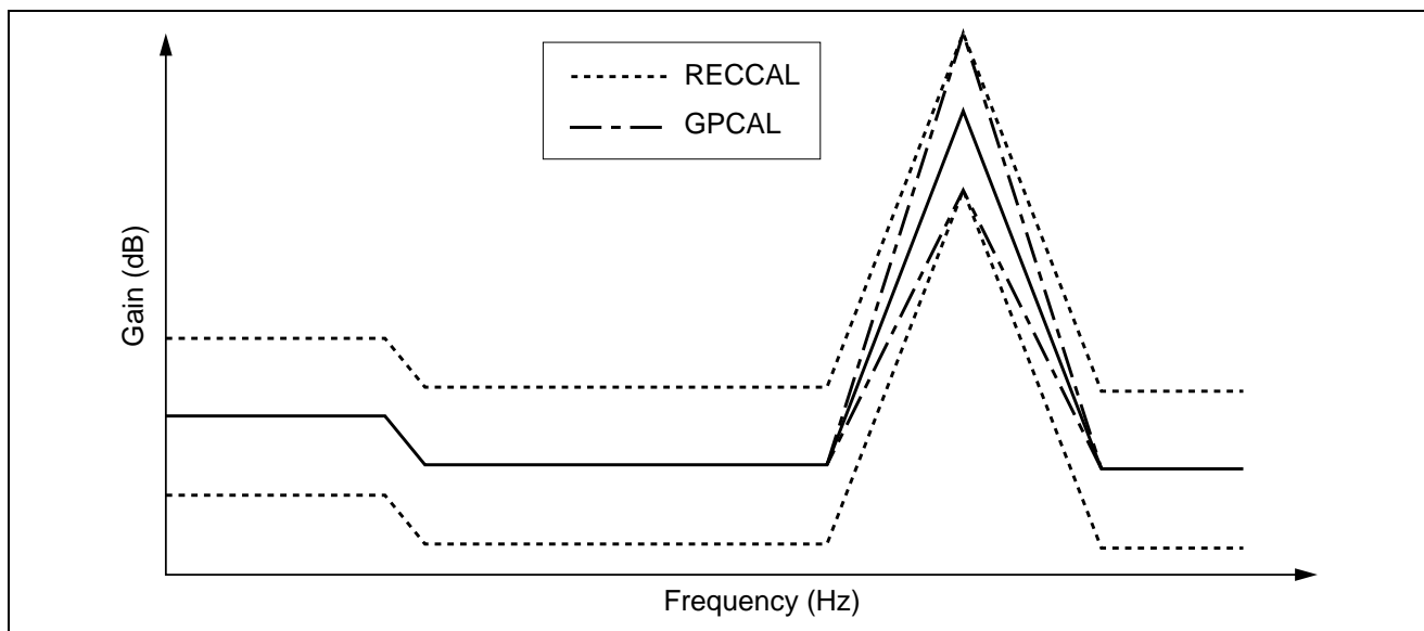
Figure 9 Frequency Characteristics of REC Equalizer
