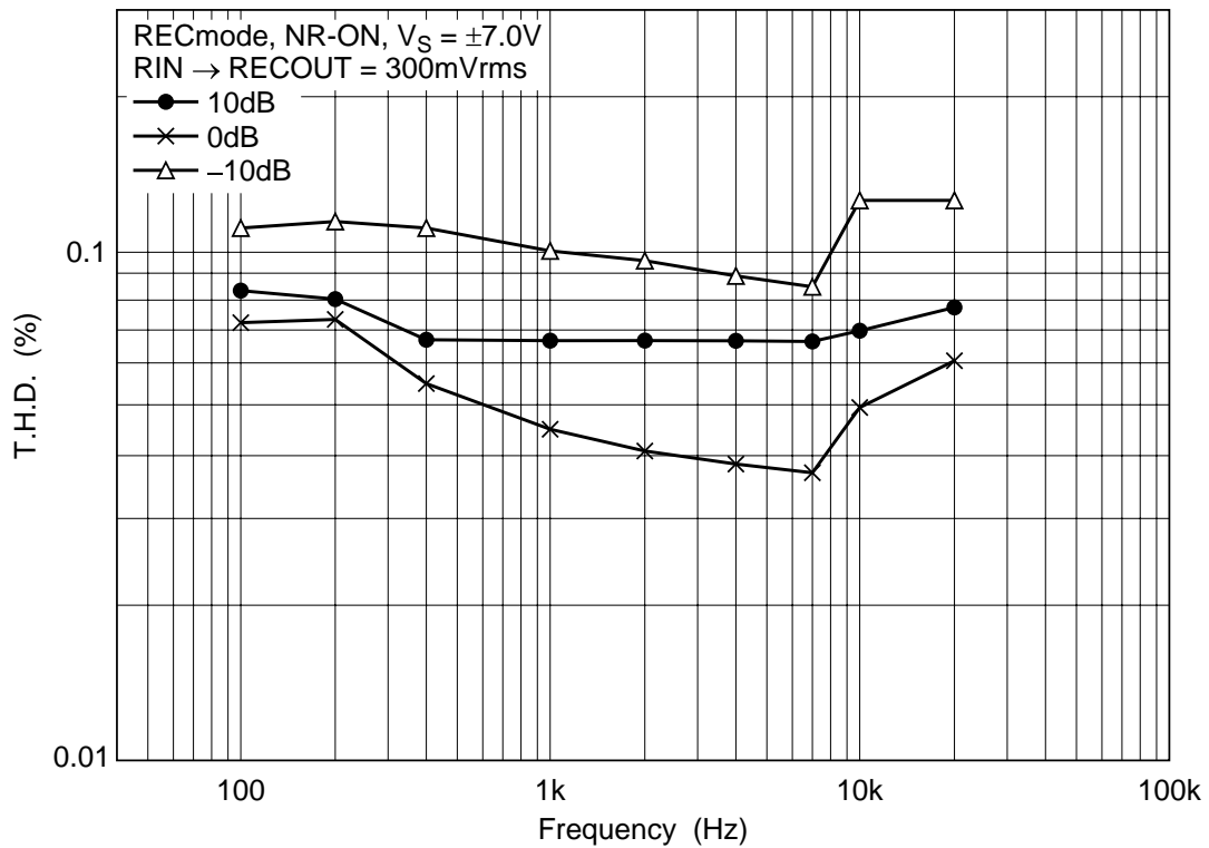
Total Harmonic Distortion vs. Frequency (2)
