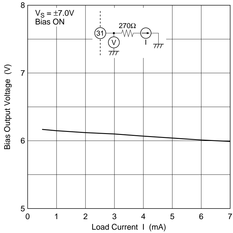
Bias Output Voltage vs. Load Current
