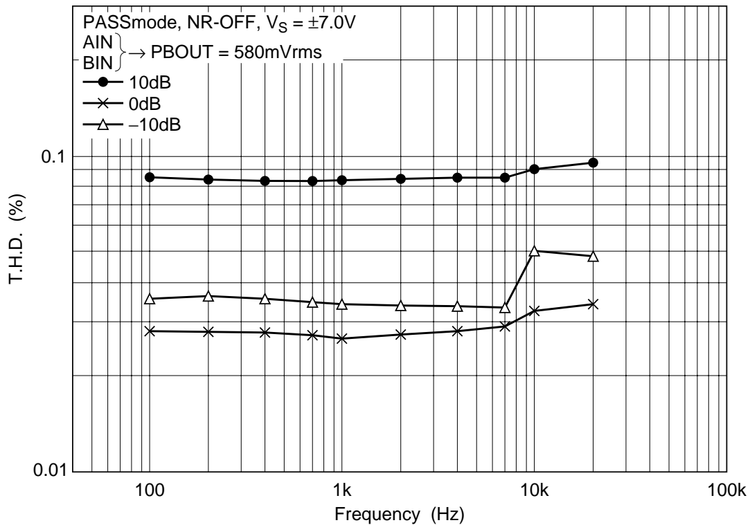
Total Harmonic Distortion vs. Frequency (5)
