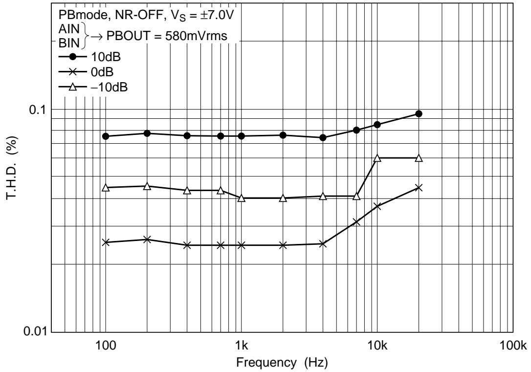
Total Harmonic Distortion vs. Frequency (3)
