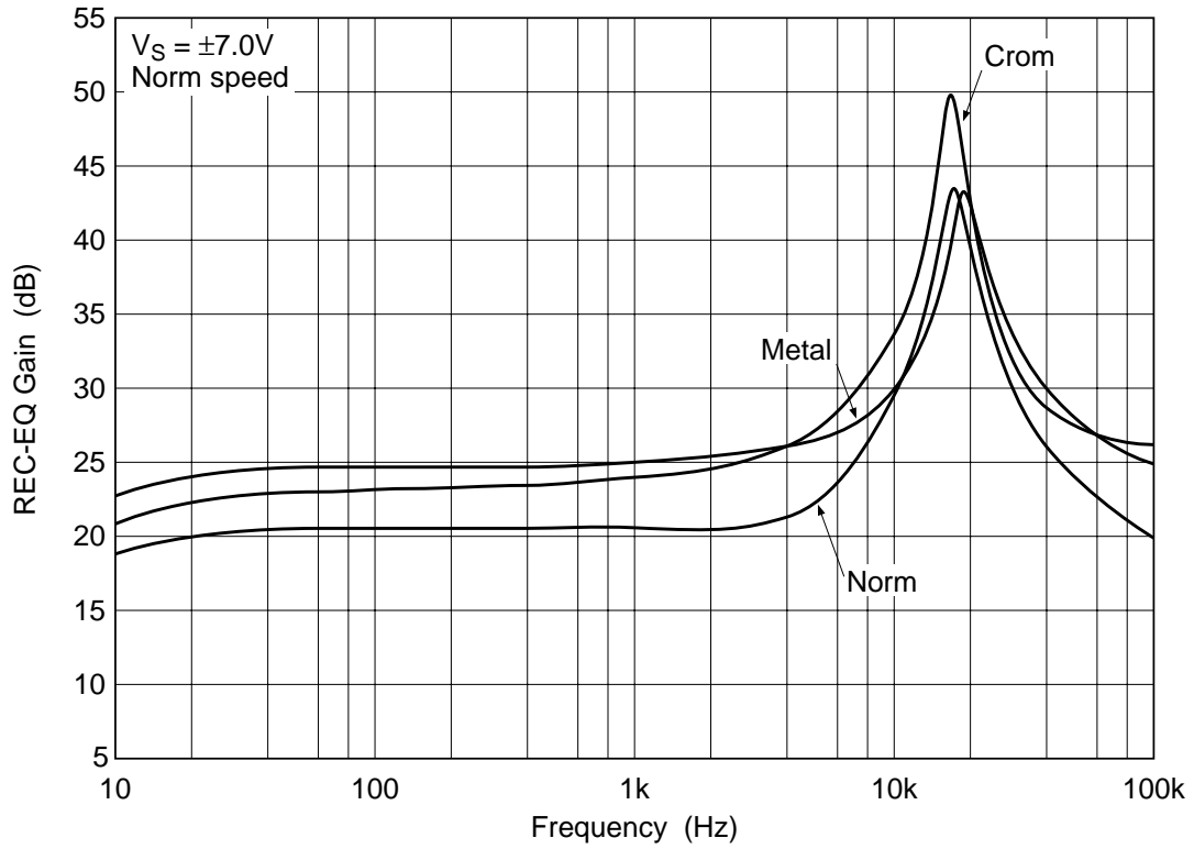
Equalizer Amp. Gain vs. Frequency (1)
