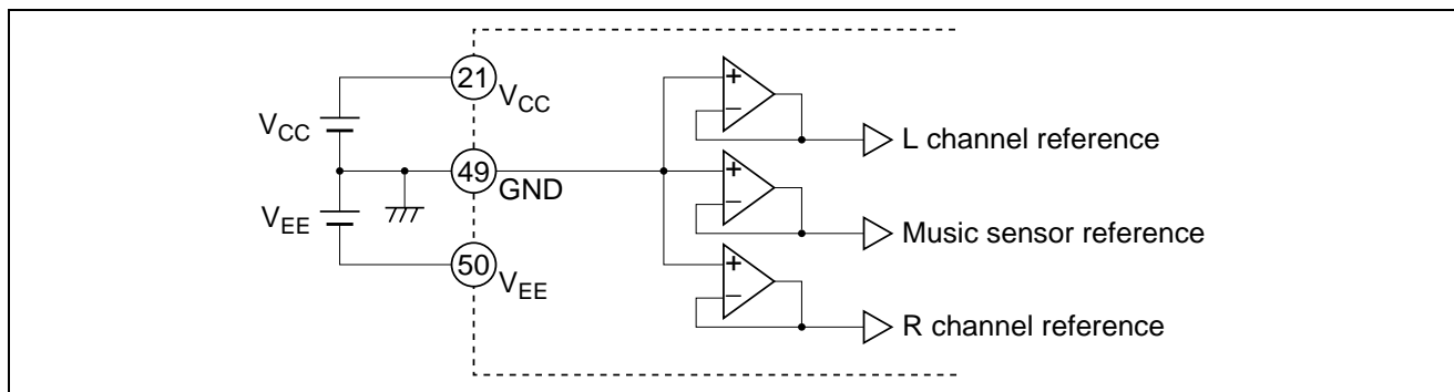
Figure 1 Reference Voltage
