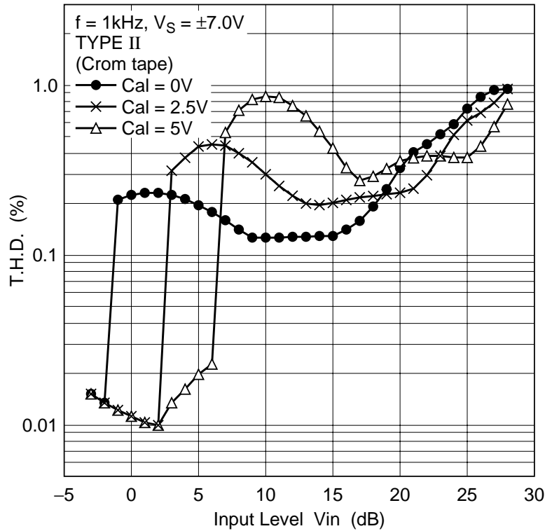
ALC Total Harmonic Distortion vs. Input Level (2)
