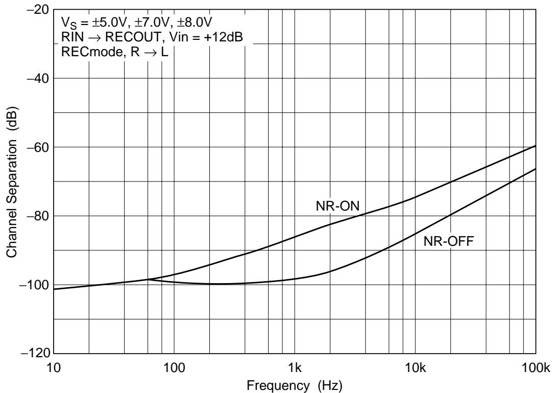
Channel Separation vs. Frequency (R→L) (1)
