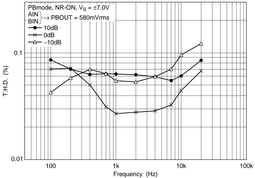
Total Harmonic Distortion vs. Frequency (4)
