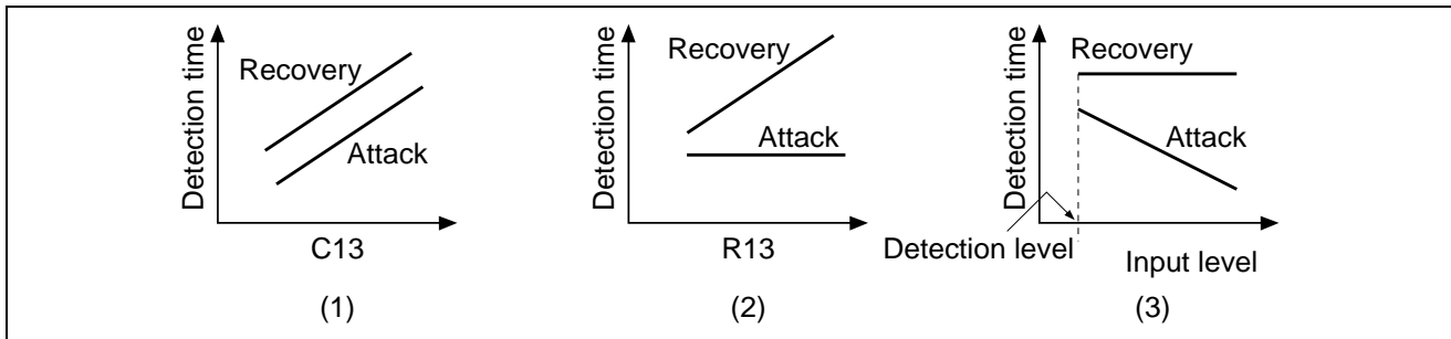
Figure 6 Function Characteristic of MS
