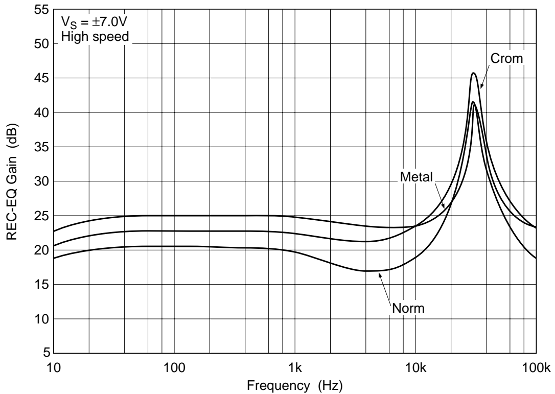
Equalizer Amp. Gain vs. Frequency (2)
