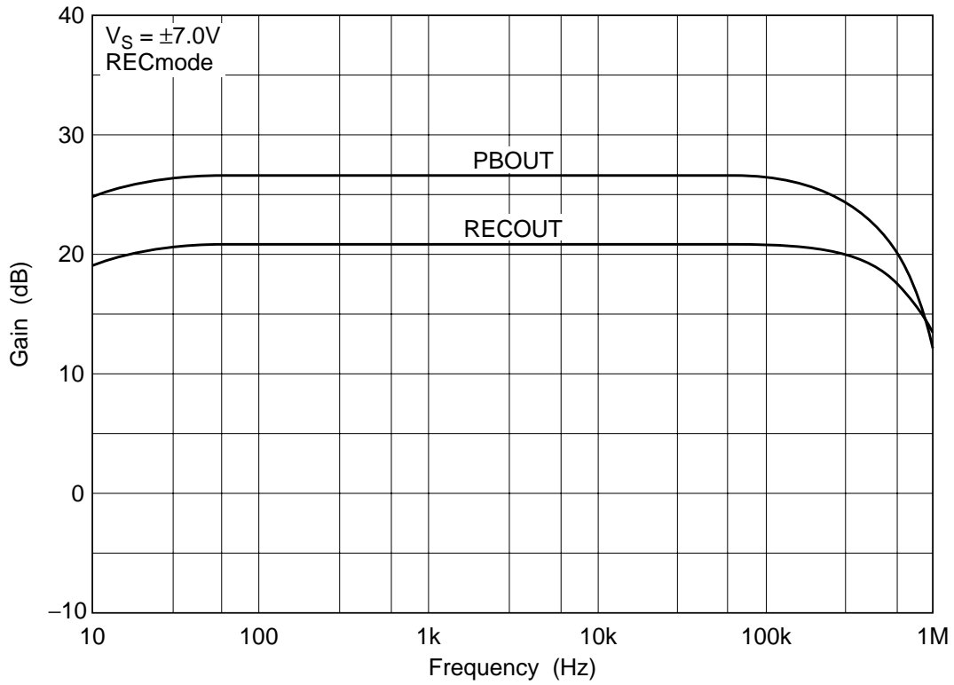
Input Amp. Gain vs. Frequency (3)
