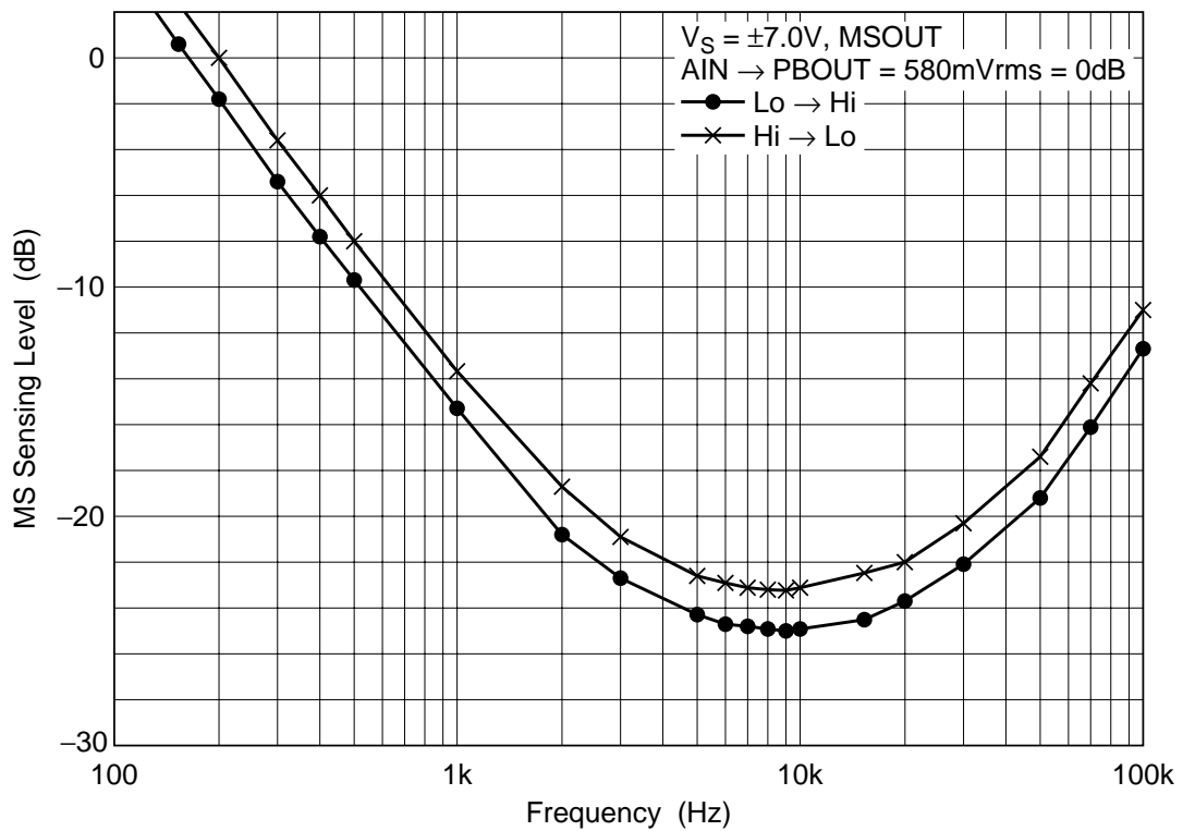
MS Sensing Level vs. Frequency
