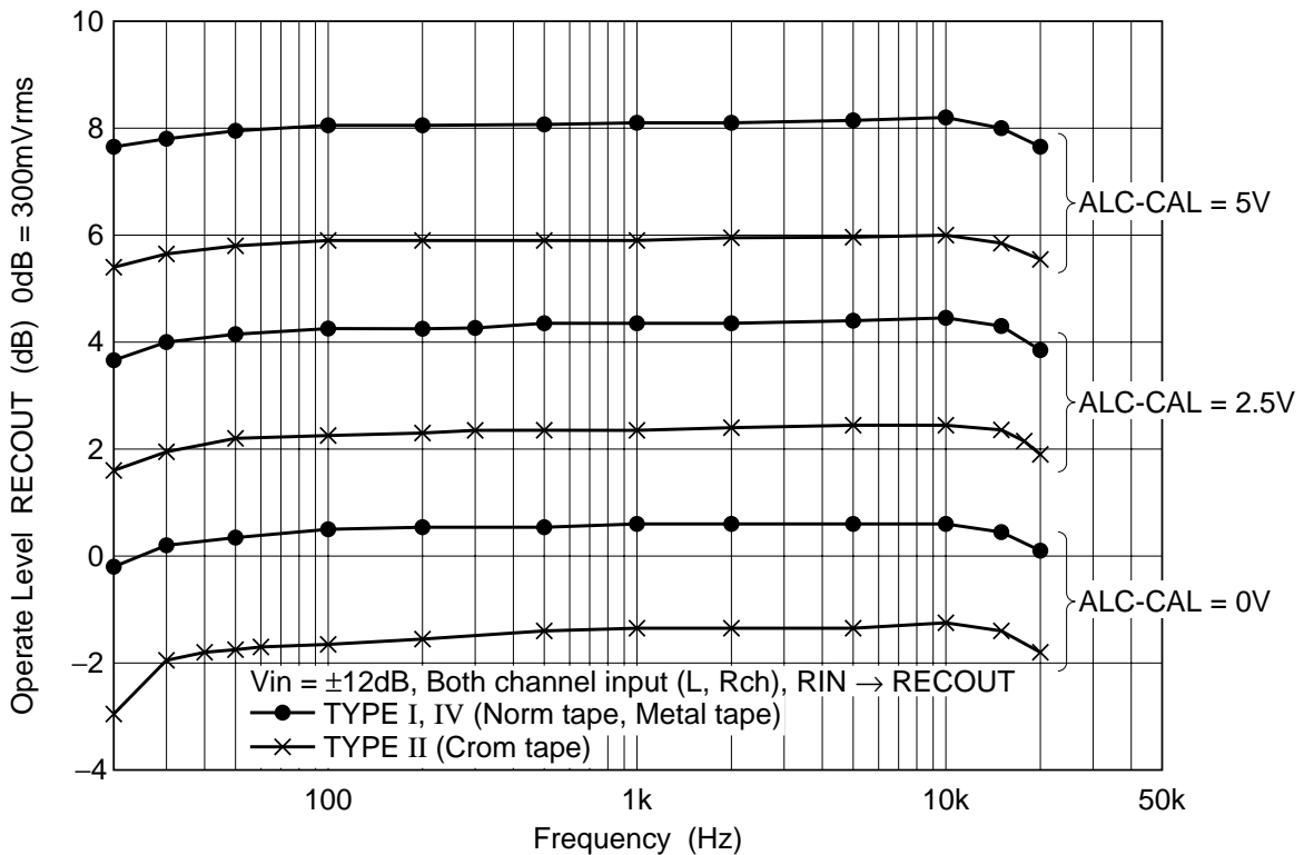
ALC Operate Level vs. Frequency
