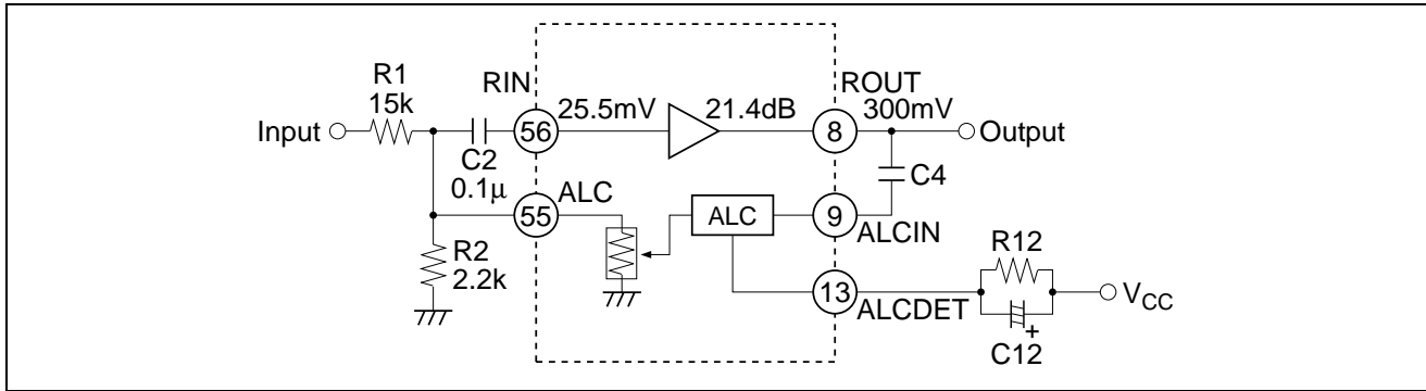
Figure 12 ALC Block Diagram
