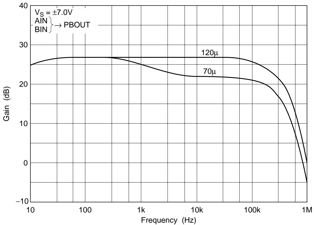
Input Amp. Gain vs. Frequency (4)
