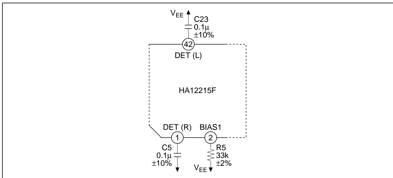
Figure 7 Tolerance of External Components
