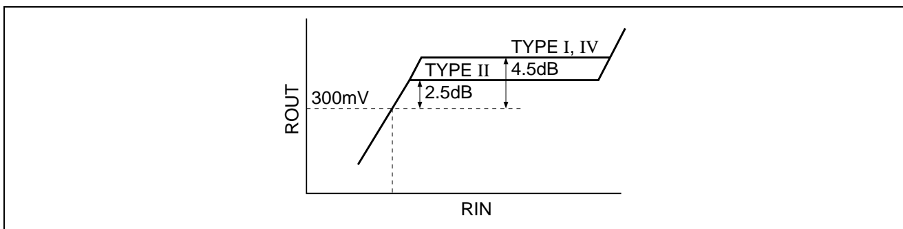
Figure 11 ALC Operation Level
