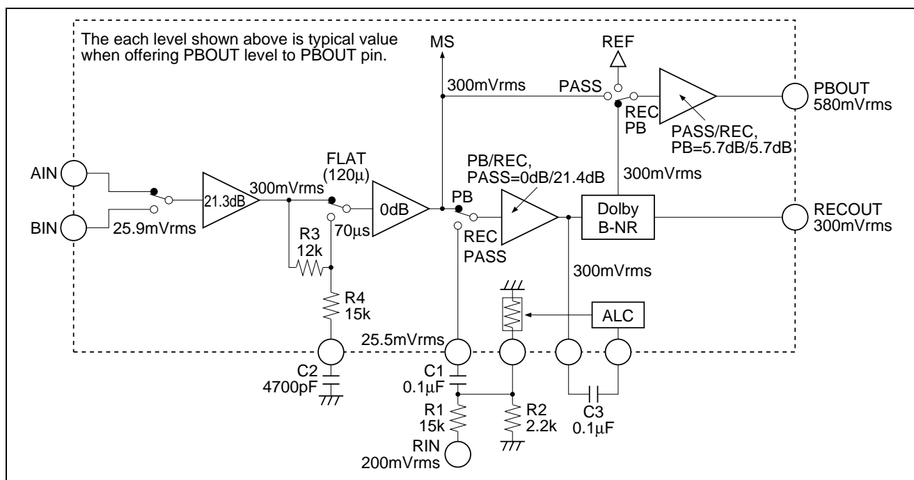
Figure 2 Input Block Diagram
