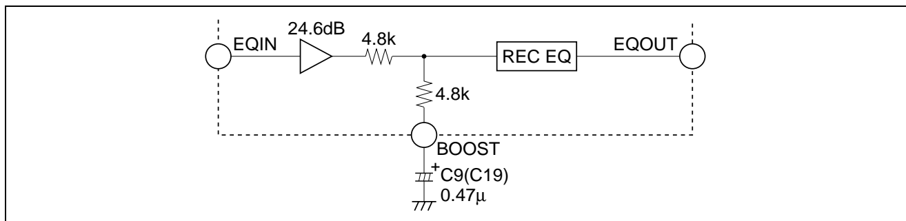
Figure 8 Example of Low Boost Circuit
