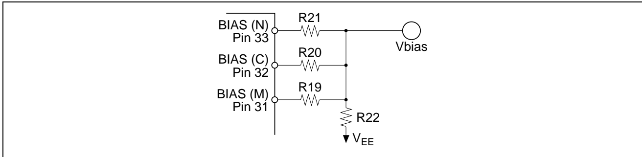
Figure 10 External Components of Bias Block
