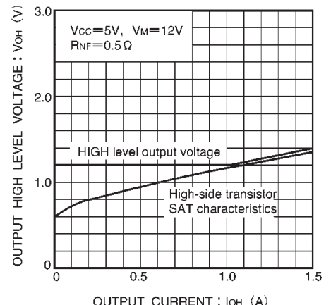
Fig.21 Output high level voltage vs. output current
