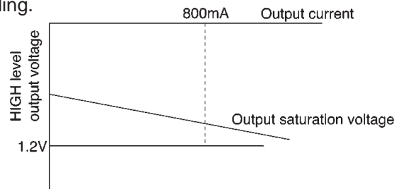
Fig.12 Transistor HIGH level output voltage
