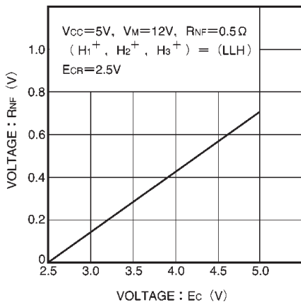
Fig.19 Output voltage vs. torque control voltage
