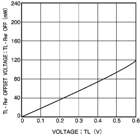
Fig.22 TL-RNF offset voltage vs. TL voltage
