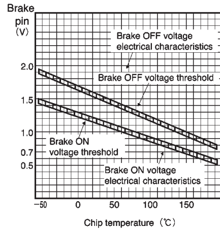
Fig.16 Brake pin threshold vs. chip temperature
