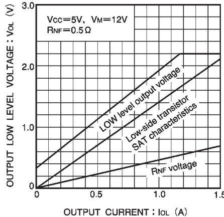
Fig.20 Output low level voltage vs. output current
