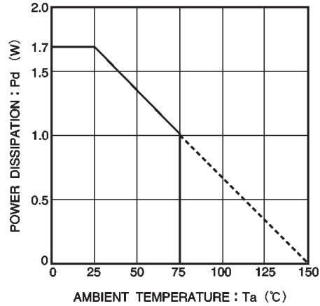
Fig.23 Power dissipation vs. ambient temperature
