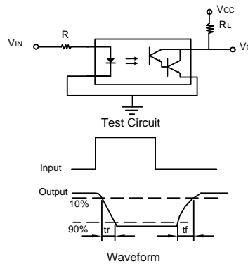
Switching Time Test Circuit
