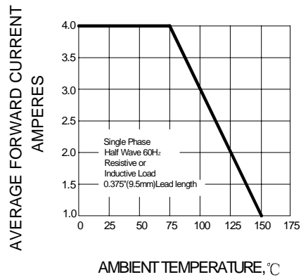
FIG.5 – FORWARD DERATING CURVE
