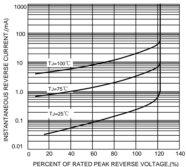
FIG.3-TYPICAL REVER CHARACTERISTICS
