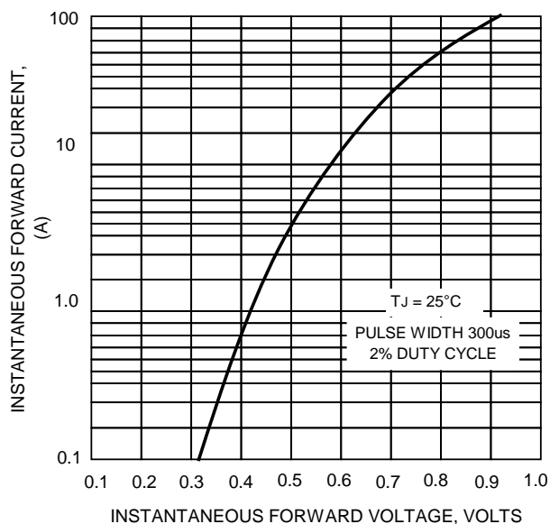
FIG.4-TYPICAL FORWARD CHARACTERISTICS
