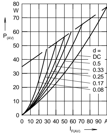
Fig. 5 Forward power loss characteristics
