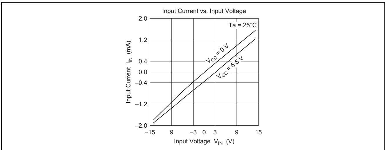
Figure 2 Input Voltage vs. Input Current Characteristics
