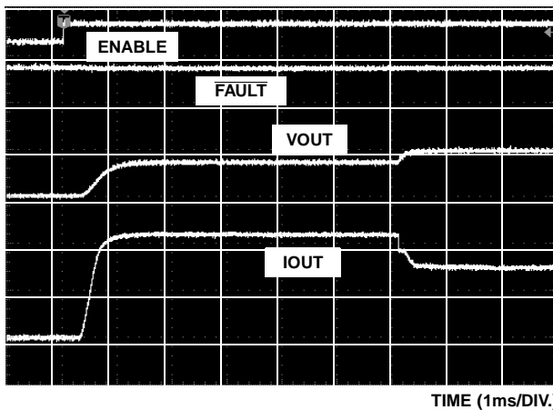
FIGURE 12. ISL6121 TURN-ON INTO A 6ms MOMENTARY OC
