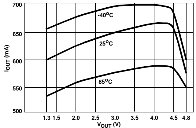
FIGURE 5. CURRENT REGULATION vs V OUT (V IN = 5V)
