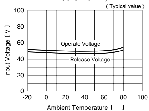
Input Characteristics VS Ambient Temperature ( S1C-245ADV )
