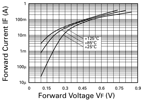
I_F v V_F Characteristics
