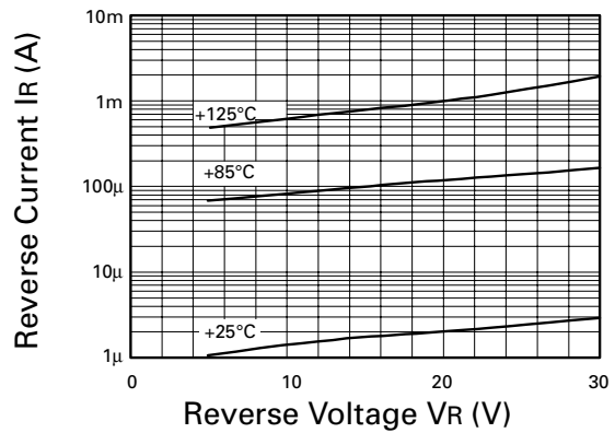
I_R v V_R Characteristics
