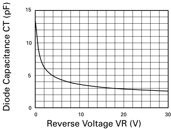
C_T v V_R Characteristics
