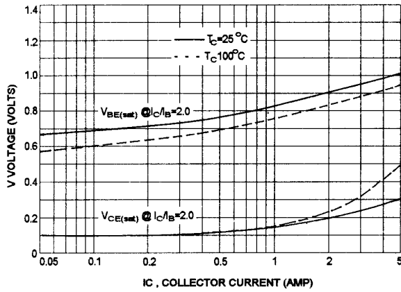
"ON" VOLTAGES
