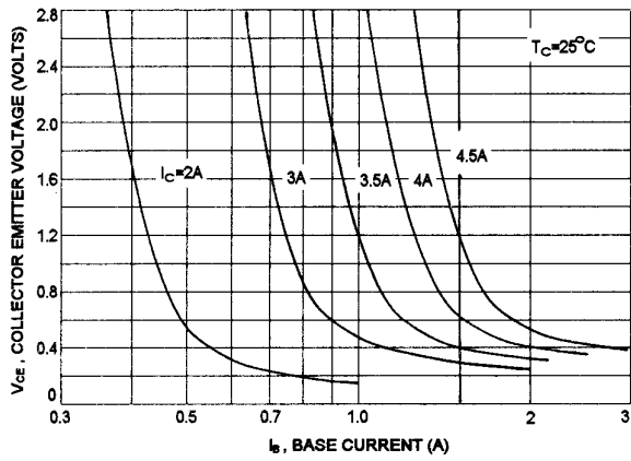
"ON" VOLTAGES
