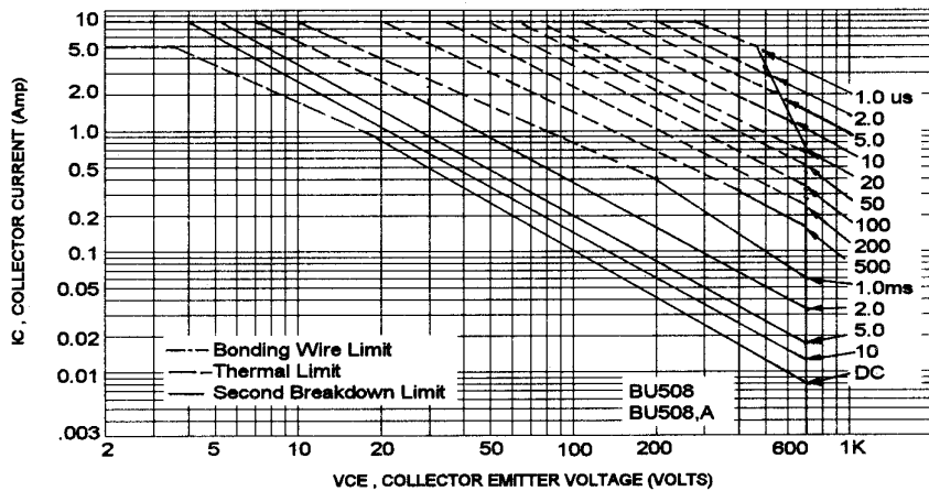
FORWARD BIAS SAFE OPERATING AREA
