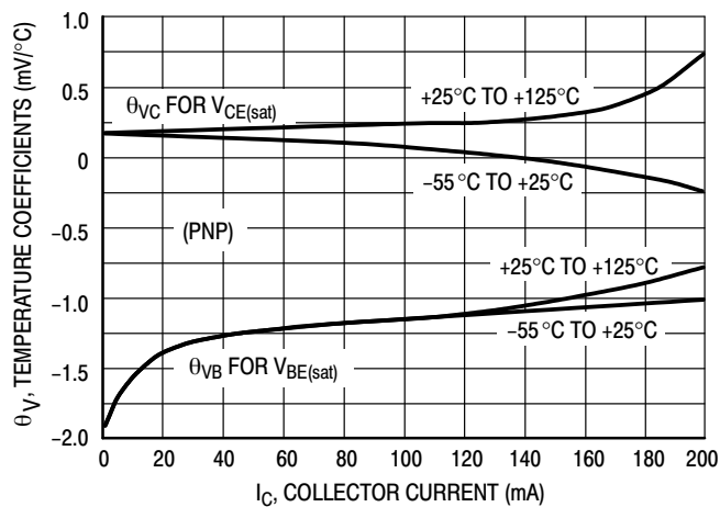
Figure 34. Temperature Coefficients
