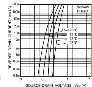
Fig.16 Reverse drain current vs. source-drain voltage ( I )
