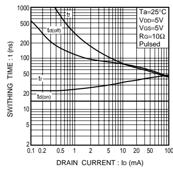
Fig.19 Switching characteristics
