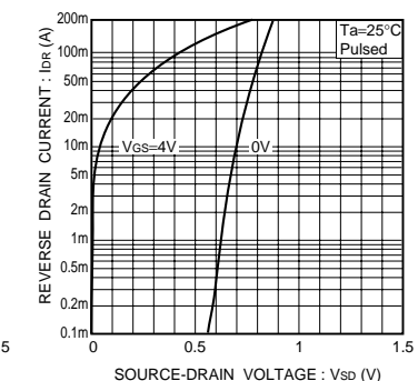
Fig.17 Reverse drain current vs. source-drain voltage ( II )
