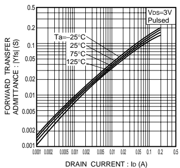
Fig.15 Forward transfer admittance vs. drain current
