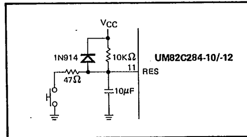
Figure 2. Typical RC RES Timing Circuit
