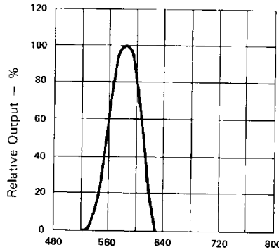
Fig 2 SPECTRAL RESPONSE
