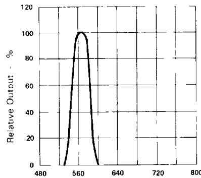
Fig 2 SPECTRAL RESPONSE
