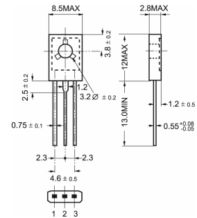
TO-126
