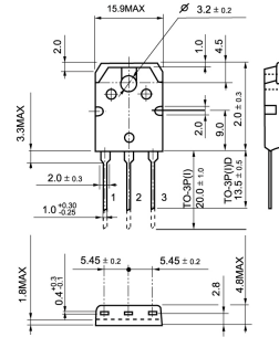
TO-3P(I)D
