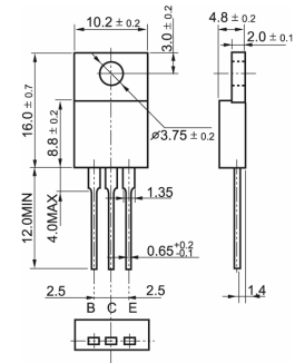
TO-220
