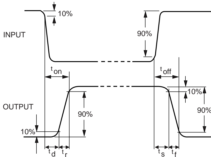
Fig. 1 Switching Waveforms
