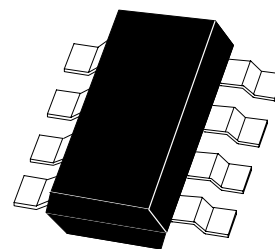
SM-8 (8 LEAD SOT223)
