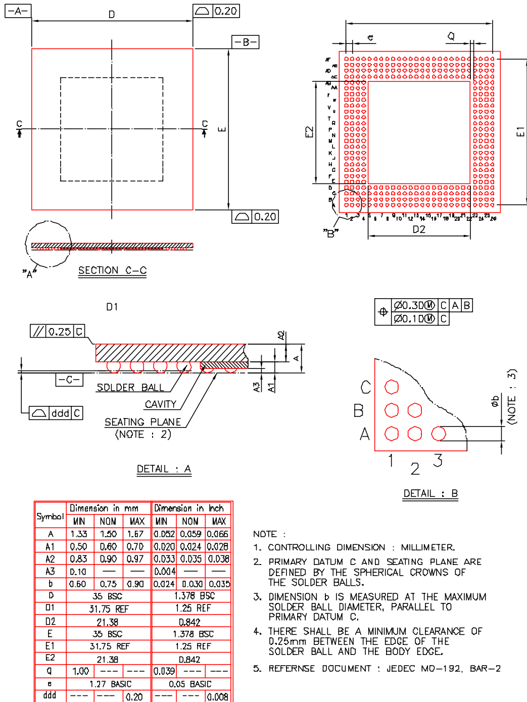
Figure 8.1 EBG352 Package
