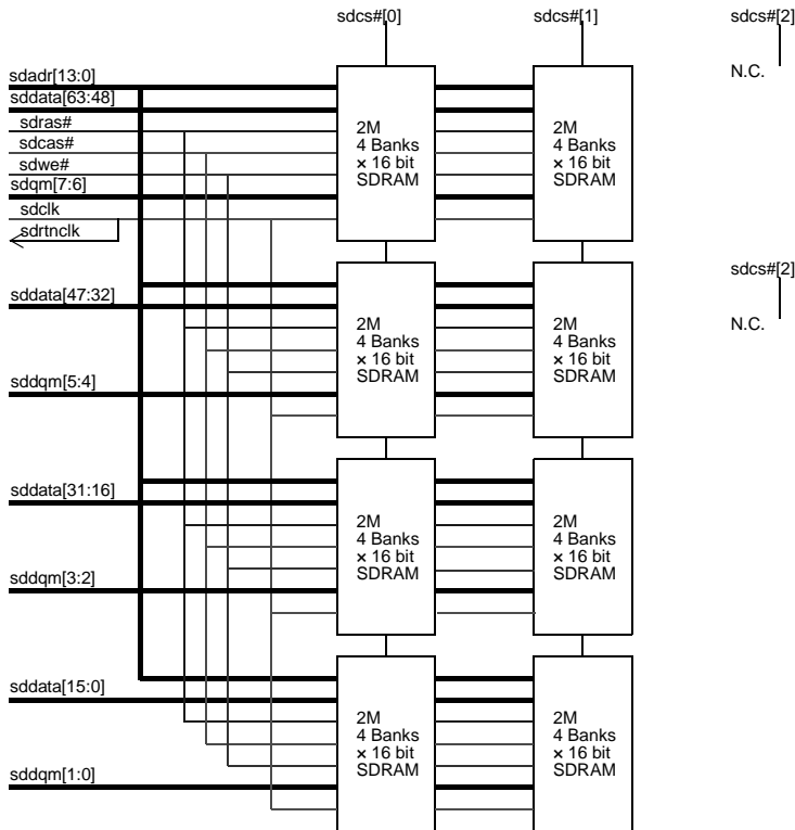
Figure 5.6 64-bit, 128 MB configuration using \times 16 , 128 Mb
