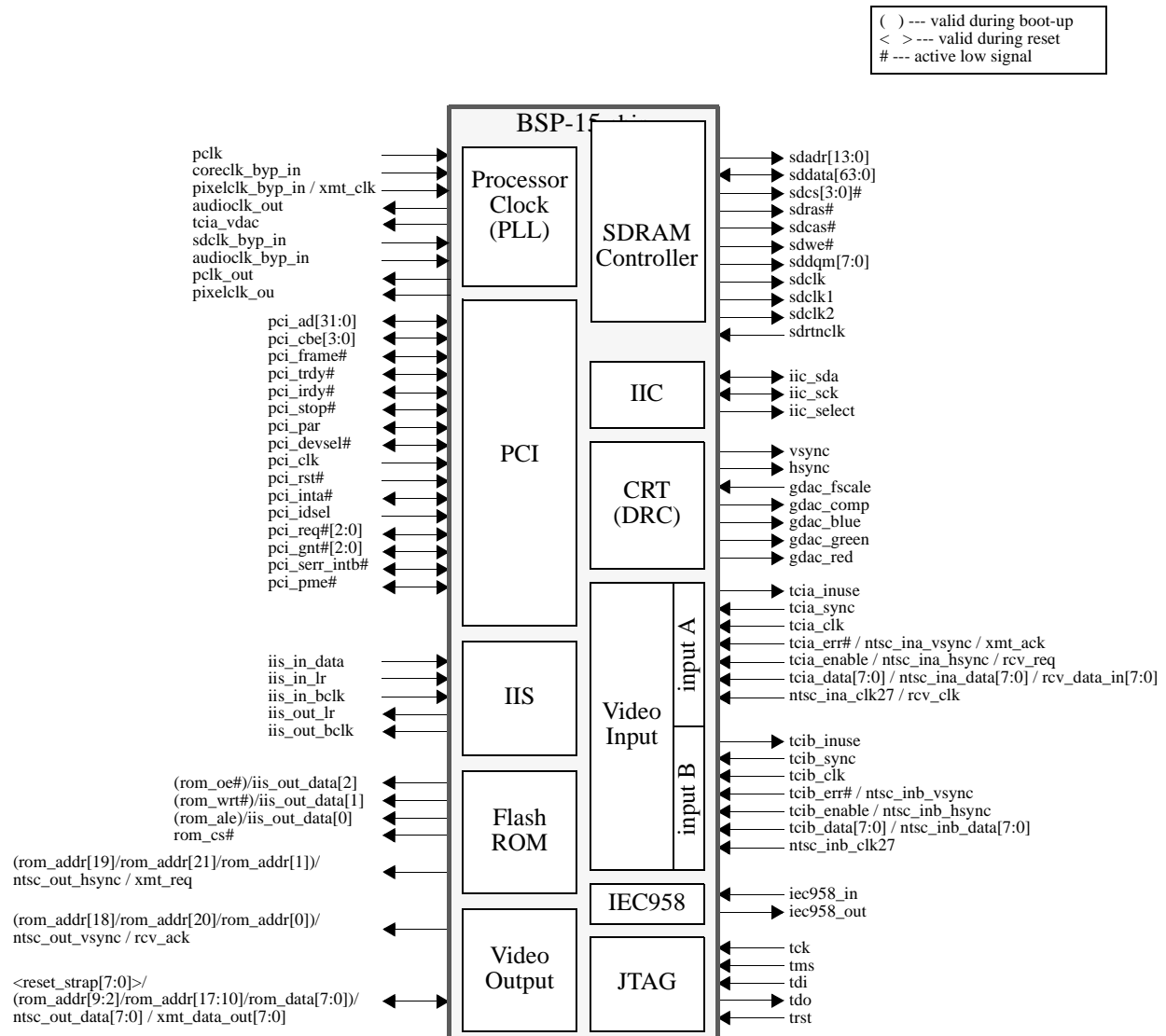
Figure 4.1 BSP-15 Interface
