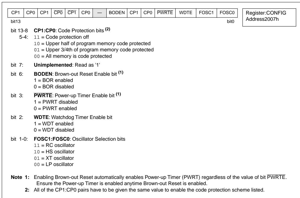
FIGURE 10-1: CONFIGURATION WORD
