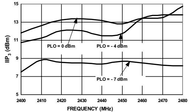
IIP_3 vs. LO Power and Frequency I_{DD} = 6.7\text{ mA} , RF_{IN} = -27\text{ dBm}
