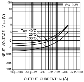
Fig.5 Input voltage vs. output current (ON characteristics)
