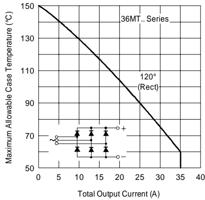
Fig. 6 - Current Ratings Characteristics
