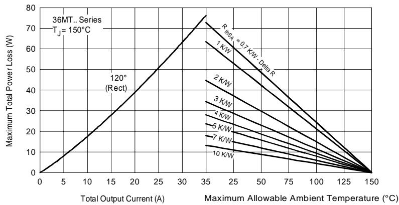
Fig. 8 - Total Power Loss Characteristics
