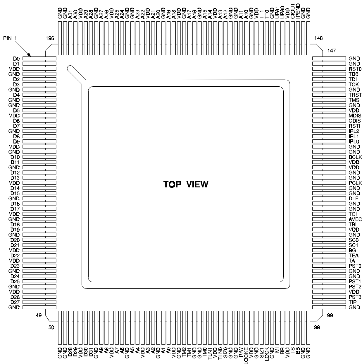
Figure 3 : Pin assignments.
