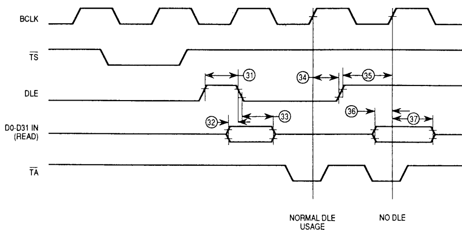
Figure 11 : DLE timing burst access.
