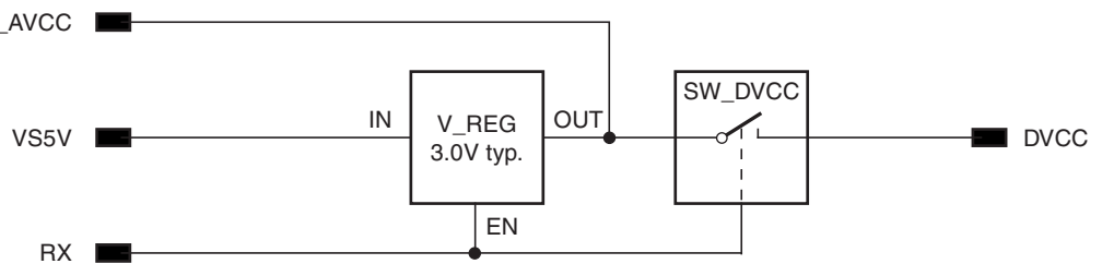
Figure 5-1. Power Supply
