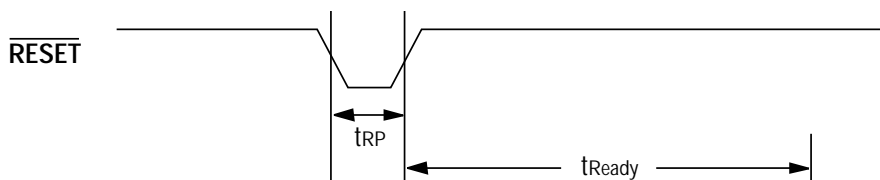
FIG. 4 RESET TIMING DIAGRAM
