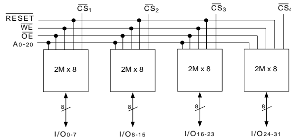
FIG. 11 ALTERNATE PIN CONFIGURATION FOR WF2M32U-XG2UX5
