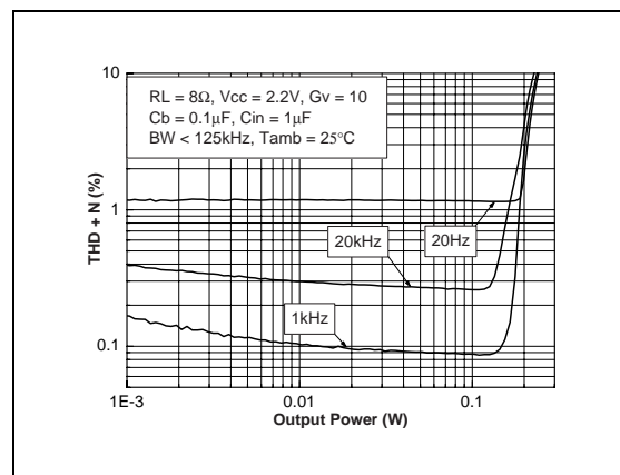
Fig. 48 : THD + N vs Output Power
