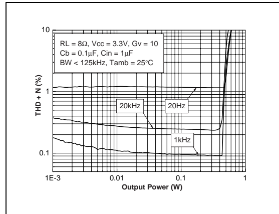
Fig. 46 : THD + N vs Output Power
