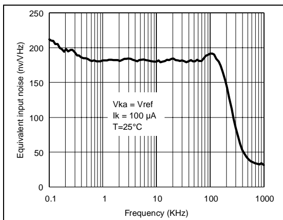
Equivalent input noise vs frequency
