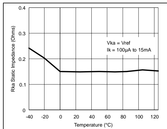
Static impedance vs temperature
