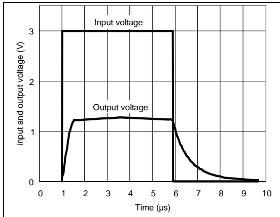
Pulse response at I_k = 1\text{mA}
