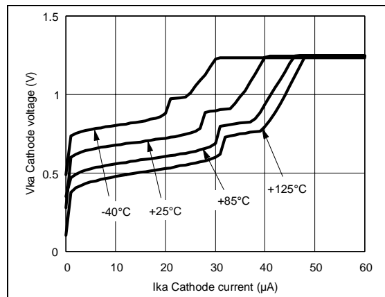
Cathode voltage vs cathode current
