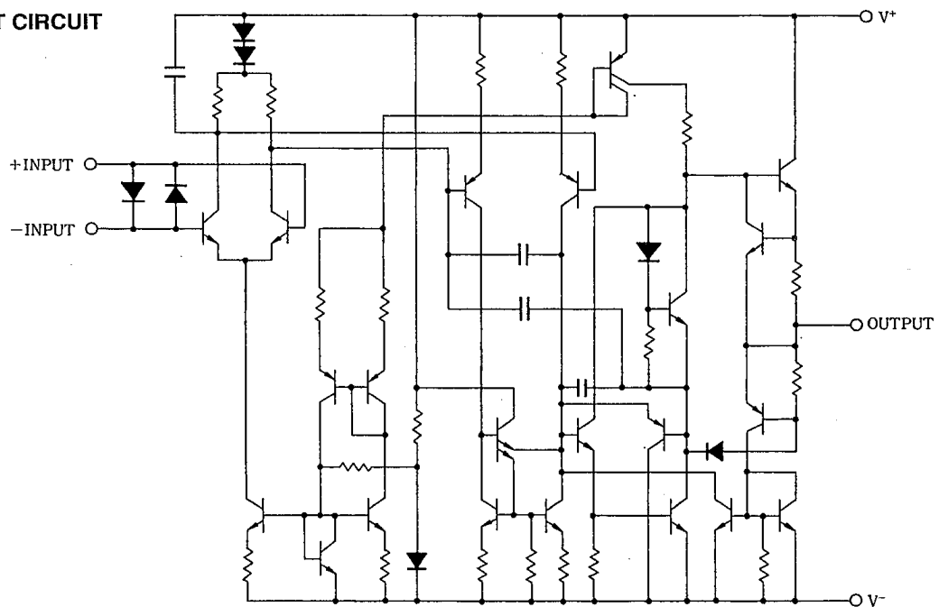
NJM5532D NJM5532M
