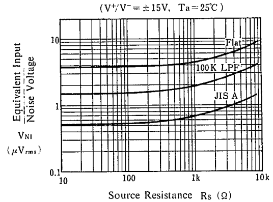
Equivalent Input Noise Voltage vs. Rs
