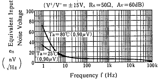
Equivalent Input Noise Voltage vs. Frequency
