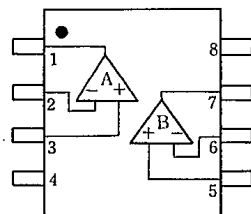
NJM5532D NJM5532M
