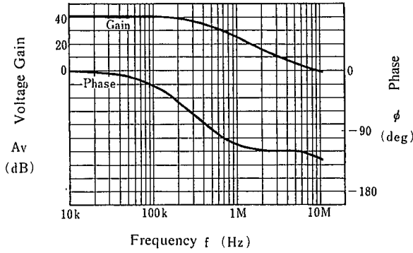
Voltage Gain, Phase vs. Frequency ( T_a = 25^\circ\text{C} )
