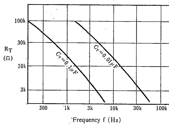
R T , C T vs. Frequency
