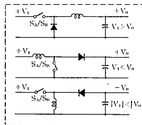
Single-Ended Inductor Circuit
