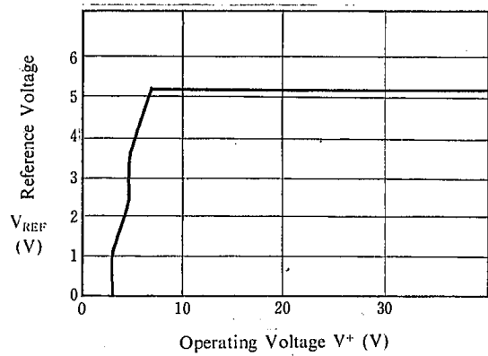
Reference Voltage vs. Operating Voltage
