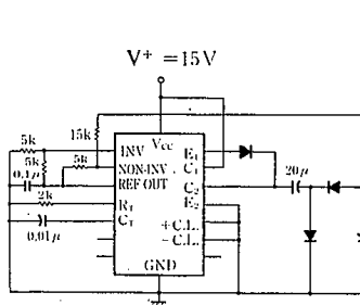
Fig. 1 Capacitor-Diode Output Circuit
