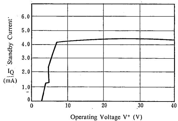
Standby Current vs. Operating Voltage
