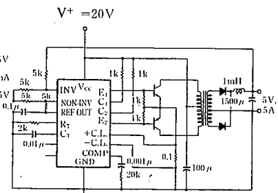
Fig. 3 Push-Pull Transformer-Coupled Circuit
