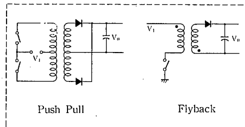
Transformer-Coupled Outputs
