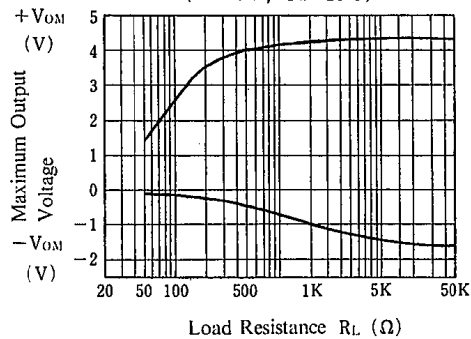
Maximum Output Voltage vs. Load Resistance
