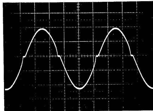
(2) Crossover Distortion Example
