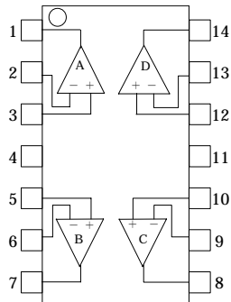
NJM13403D1/13403M NJM13403E/13403V
