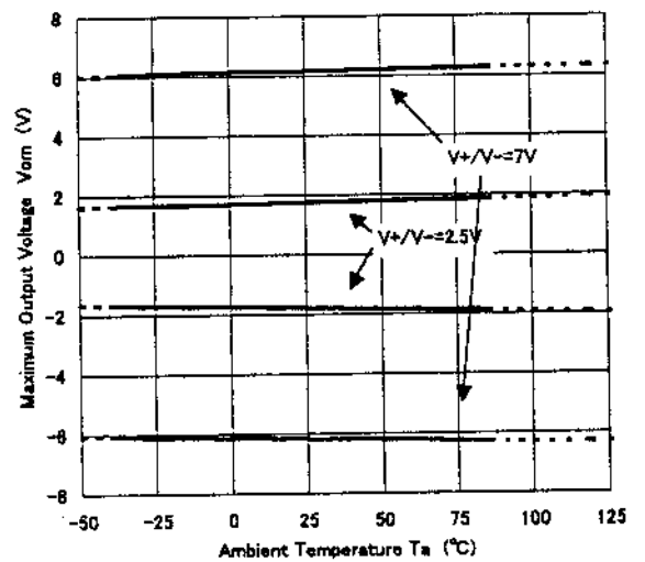
NJM13403 Maximum Output Voltage Swing vs. Temperature
