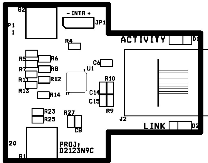
Top Silkscreen
