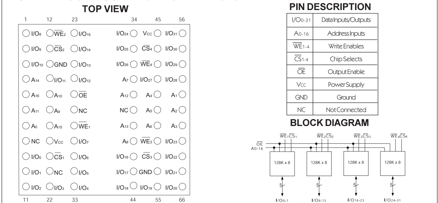
FIG. 1 PIN CONFIGURATION FOR WF128K32N-XH1X5
