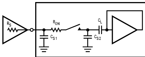
FIGURE 6. Analog Input Model
