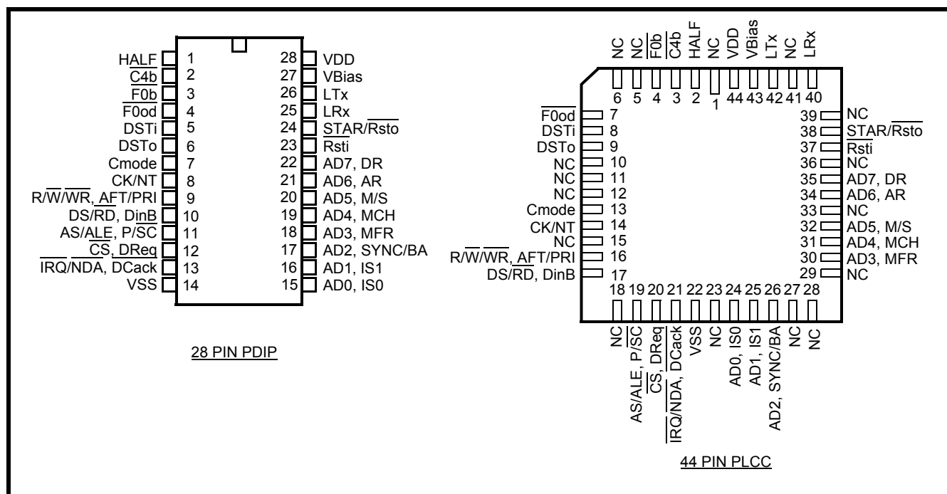
Figure 2 - Pin Connections
