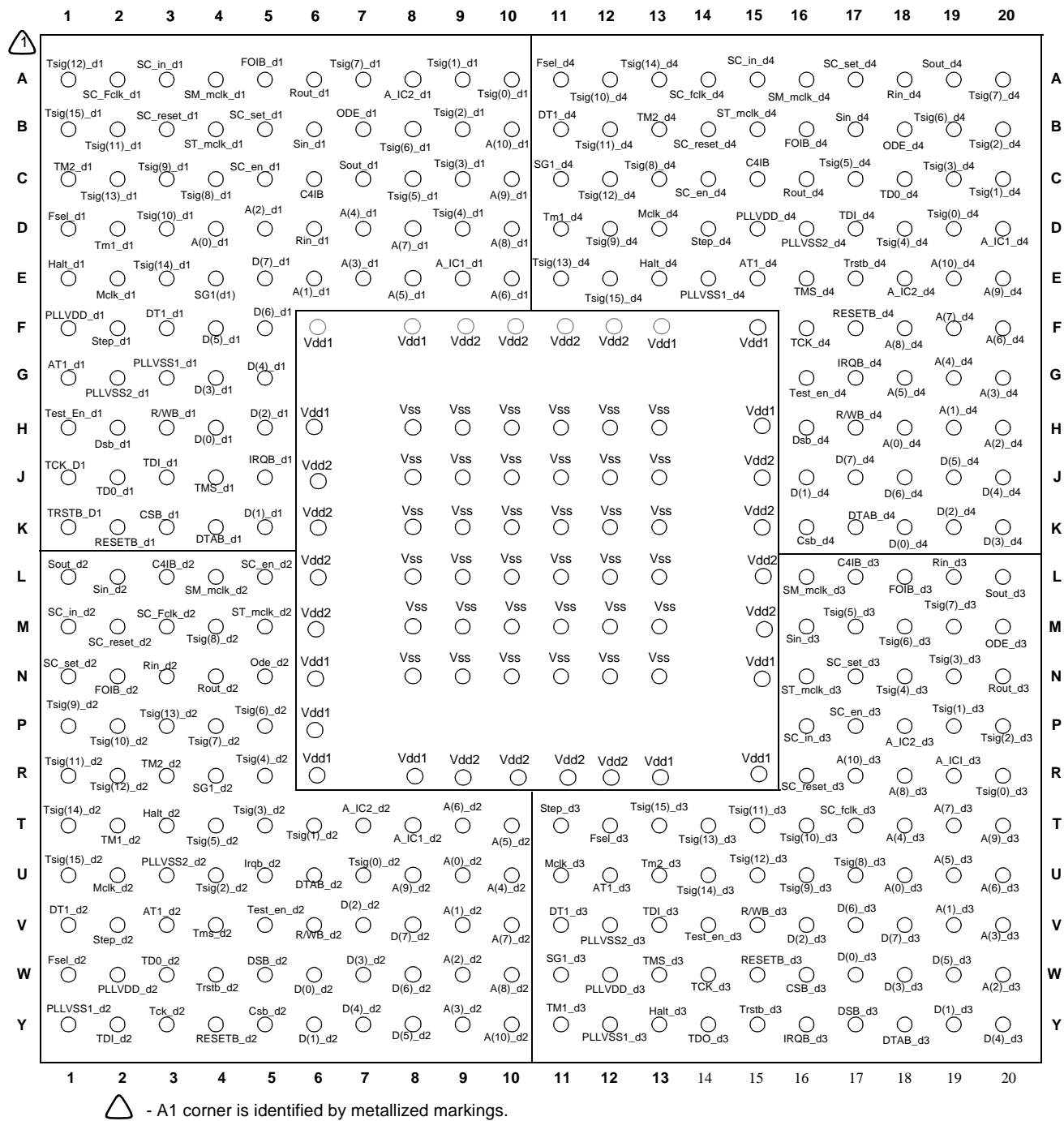
Figure 2 - 365 Ball BGA
