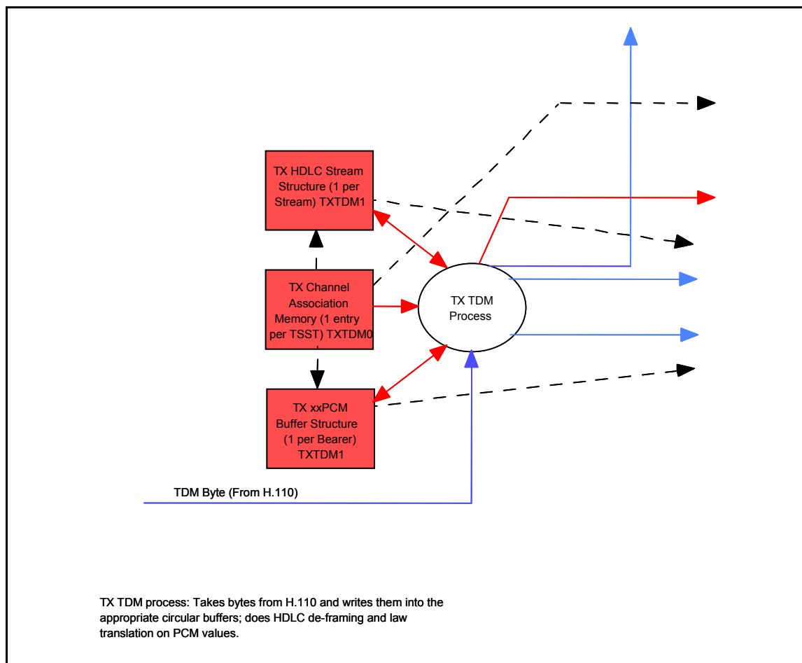
Figure 20 - Tx Flow 1
