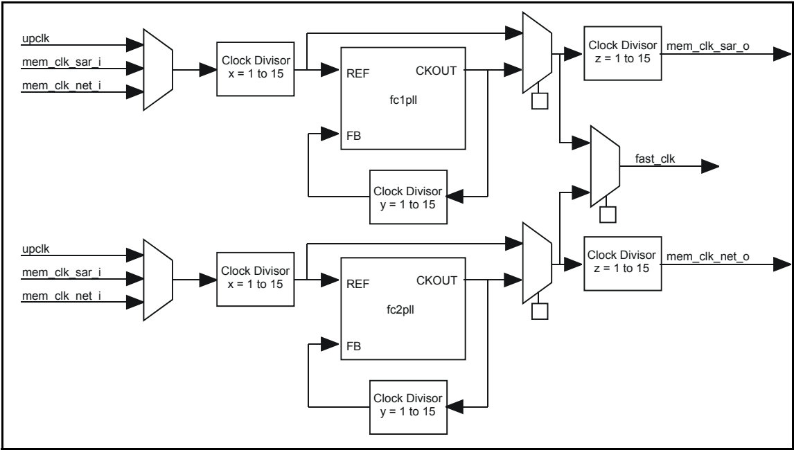
Figure 95 - Clock Synthesis
