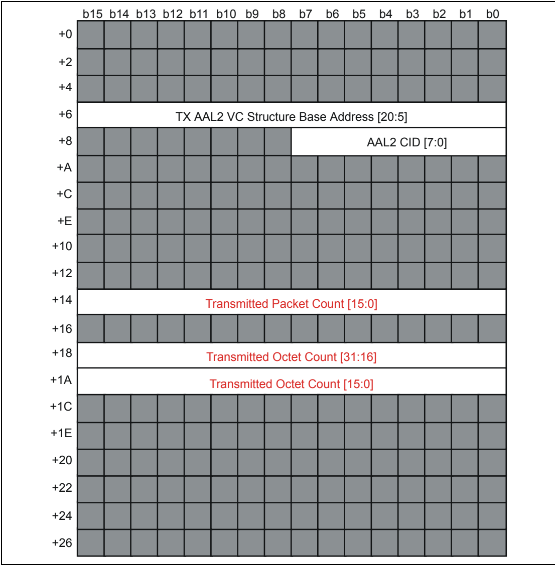
Figure 47 - TX AAL2 Connection Structure
