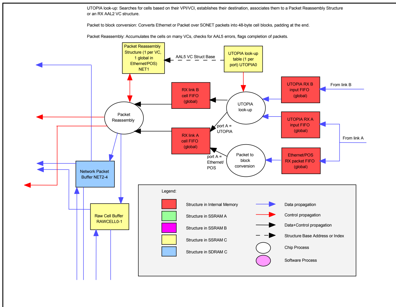
Figure 16 - Rx Flow 1
