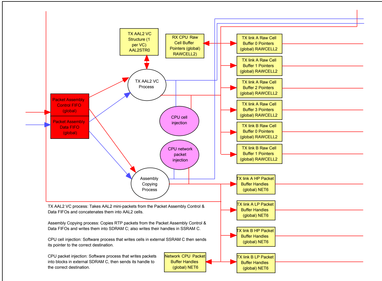
Figure 22 - Tx Flow 3
