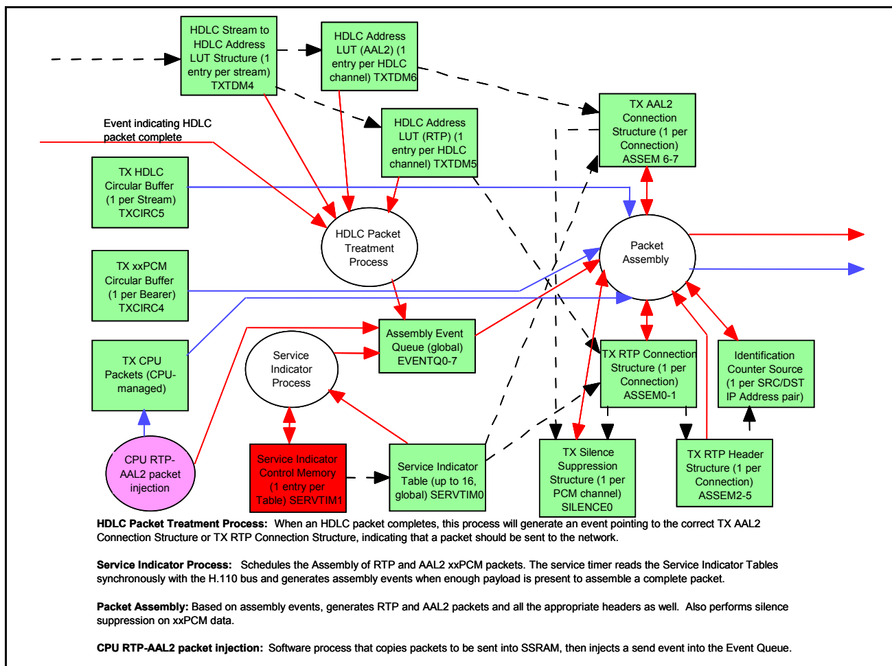
Figure 21 - Tx Flow 2
