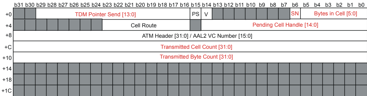
Figure 33 - TX AAL2 VC Structure
