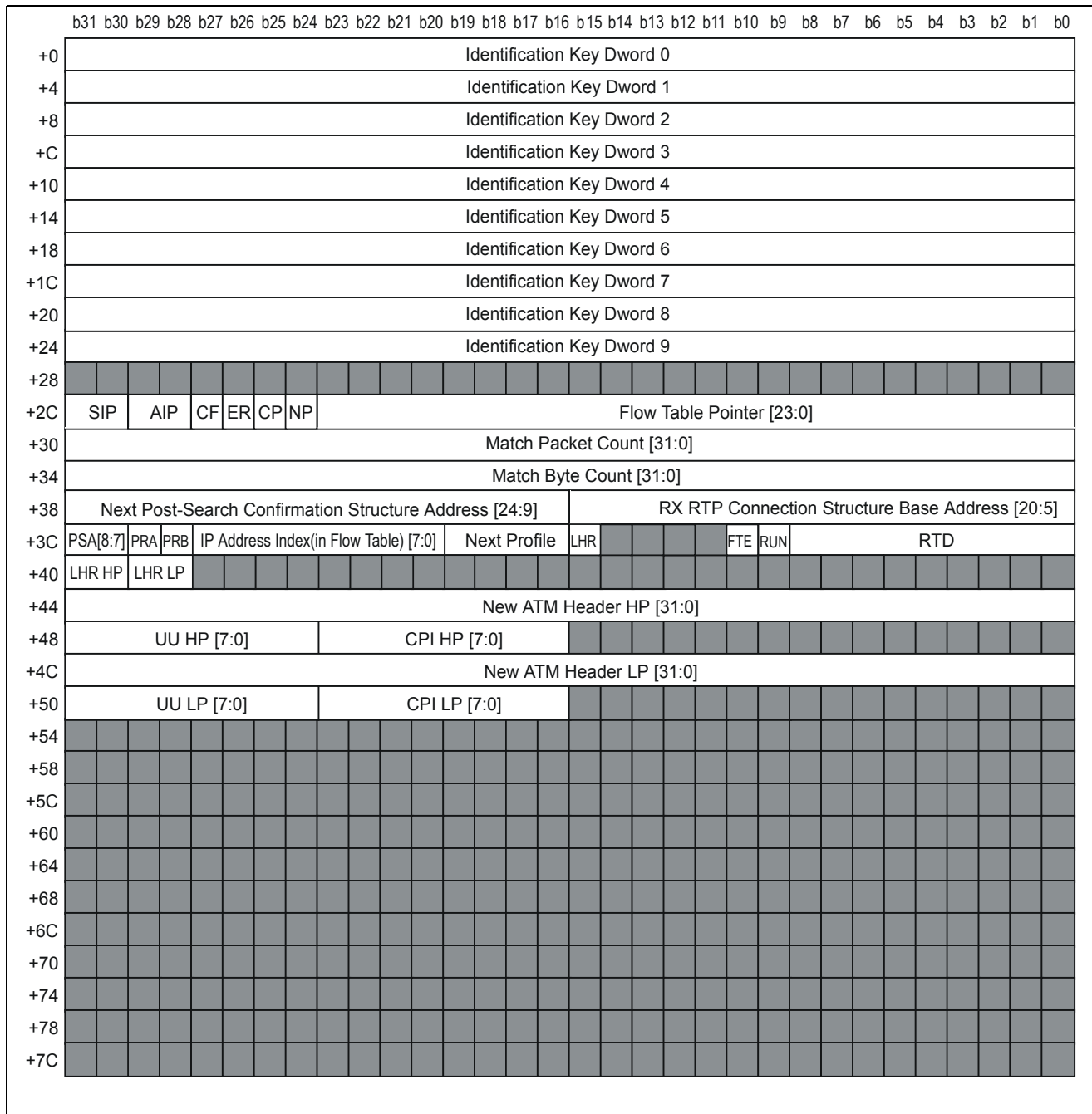
Figure 32 - Post-Search Conformation Structure
