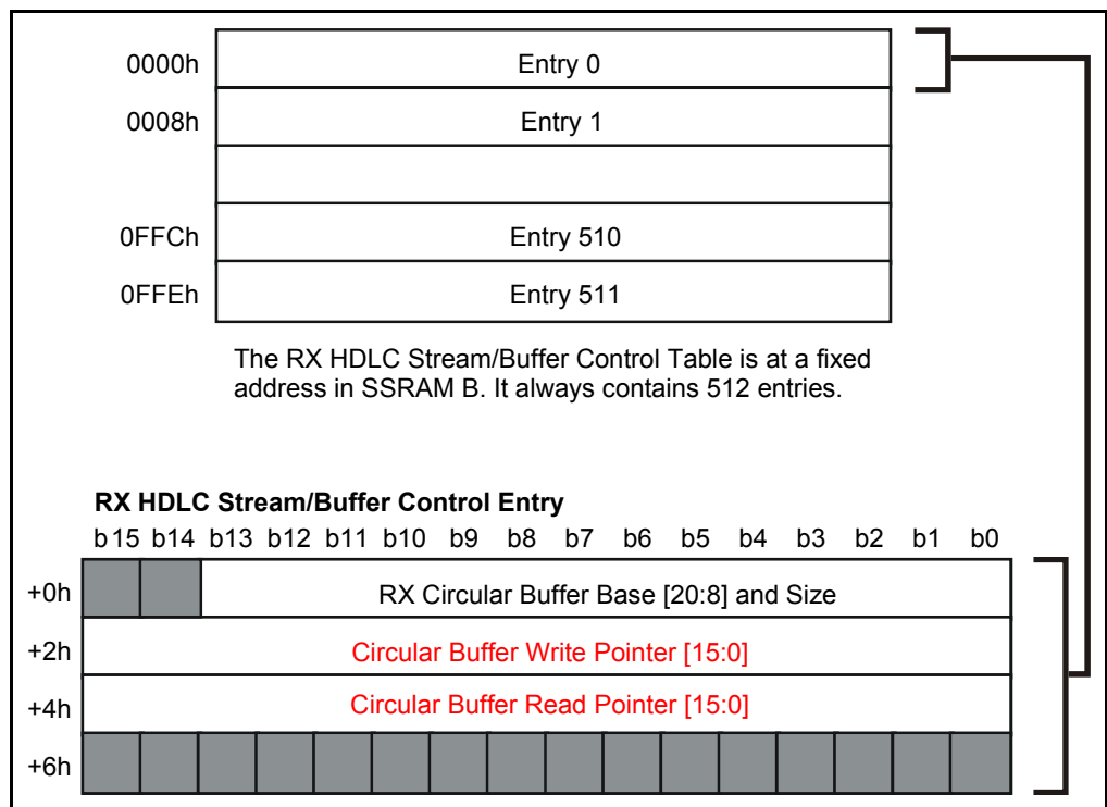
Figure 85 - RX HDLC Stream/Buffer Control Table
