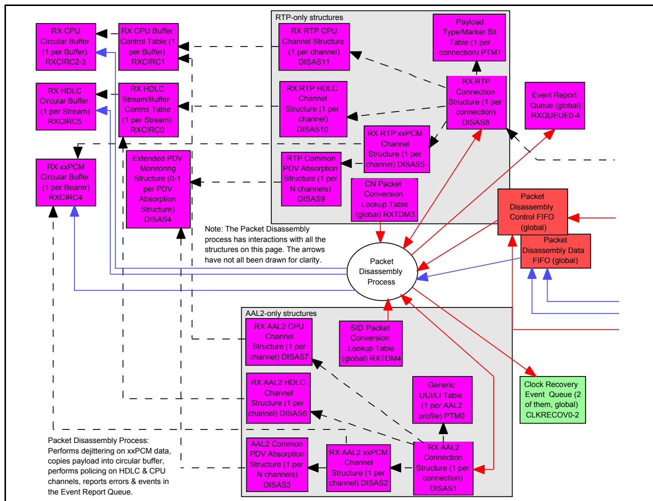
Figure 18 - Rx Flow 3
