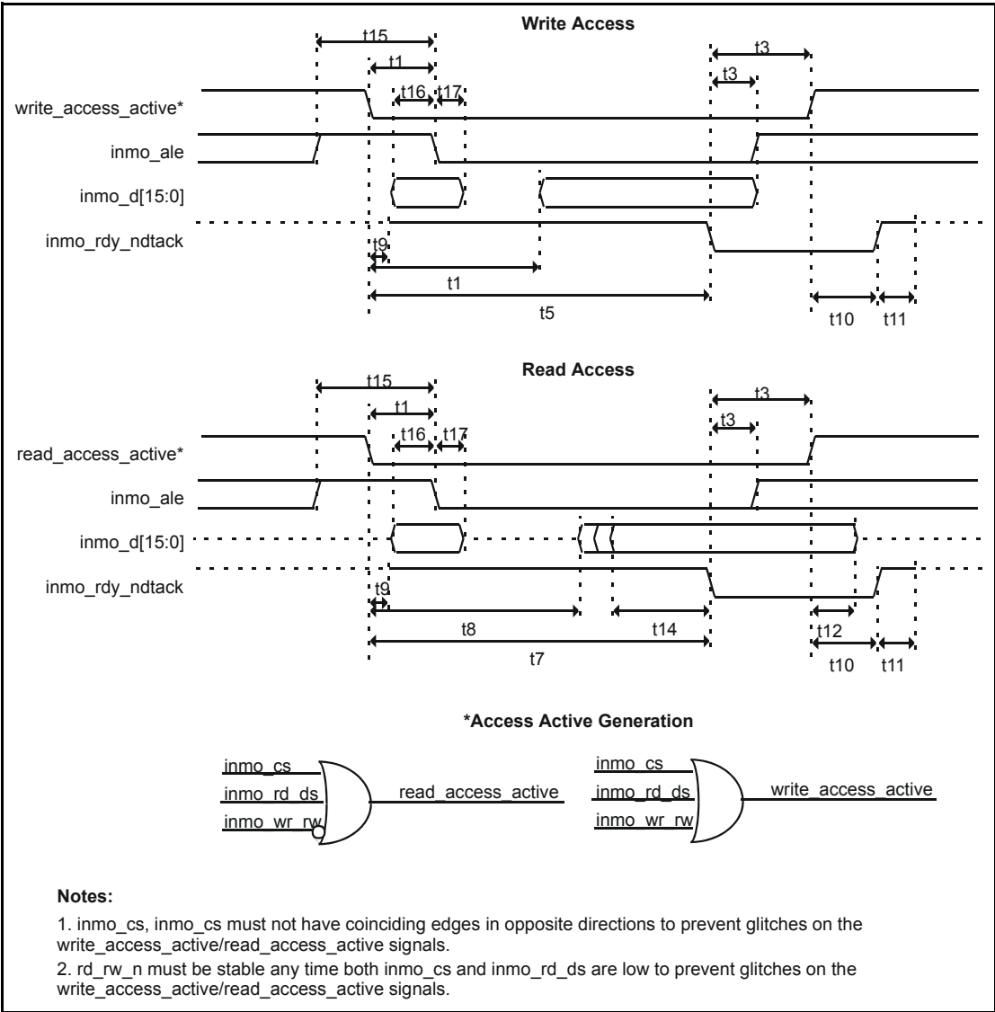
Figure 106 - Multiplexed CPU Interface - Motorola Mode
