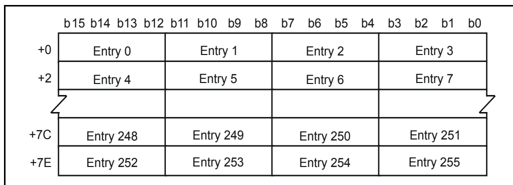
Figure 55 - Payload Type/Marker Bit Table
