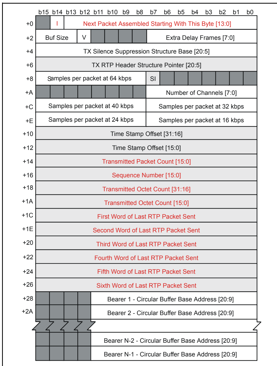
Figure 45 - xxPCM Channel Addition to TX RTP Connection Structure
