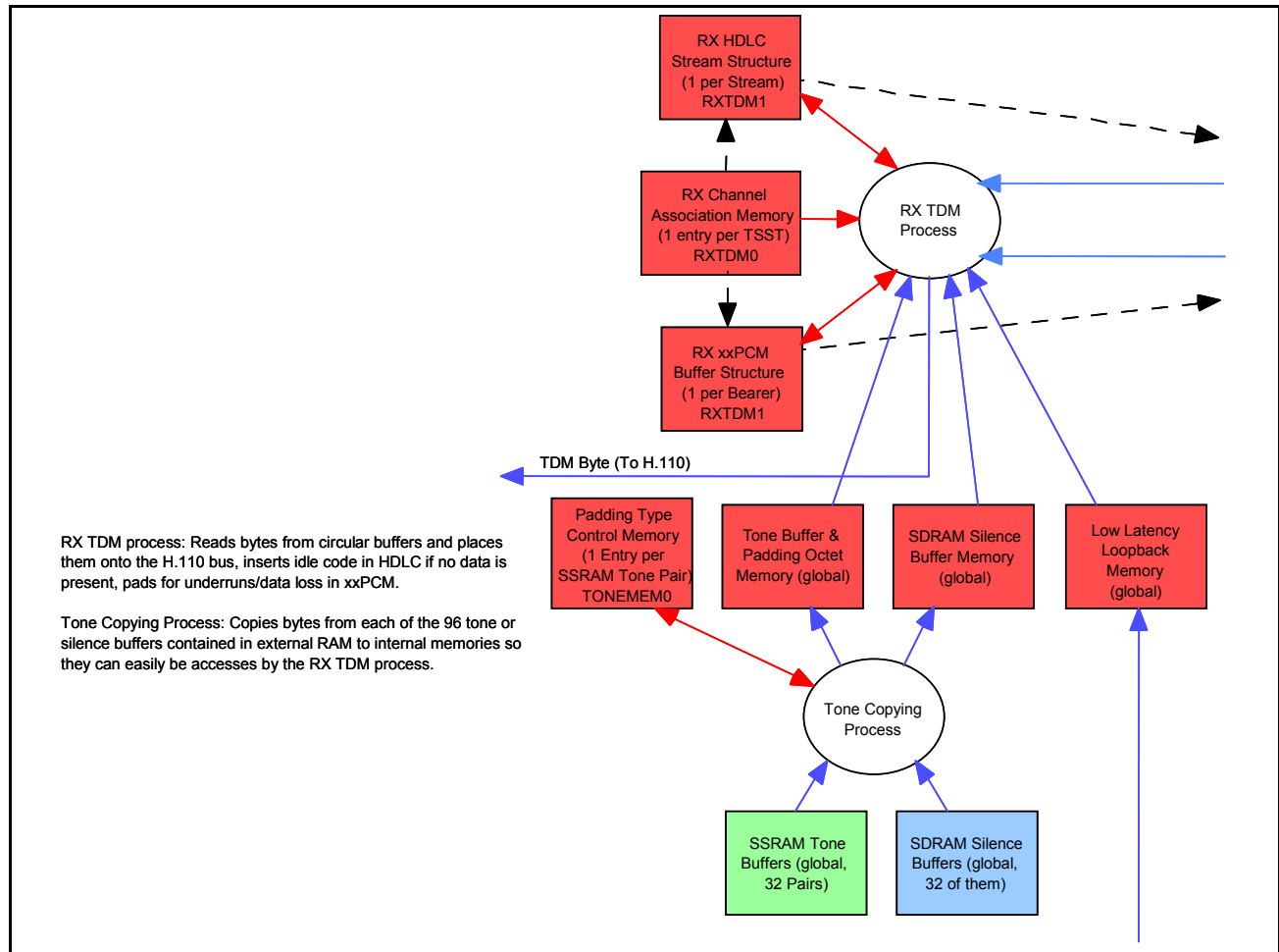
Figure 19 - Rx Flow 4
