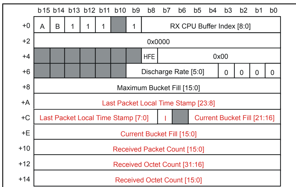
Figure 71 - RX AAL2 CPU Channel Structure
