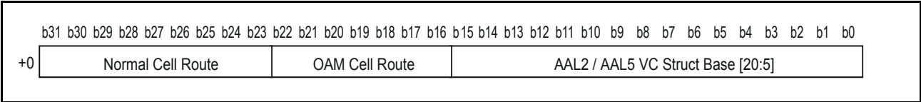
Figure 13 - UTOPIA LUT Entry Format
