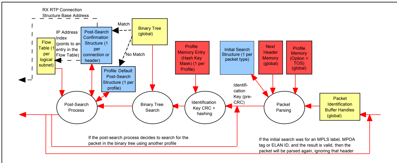
Figure 24 - Packet Identification
