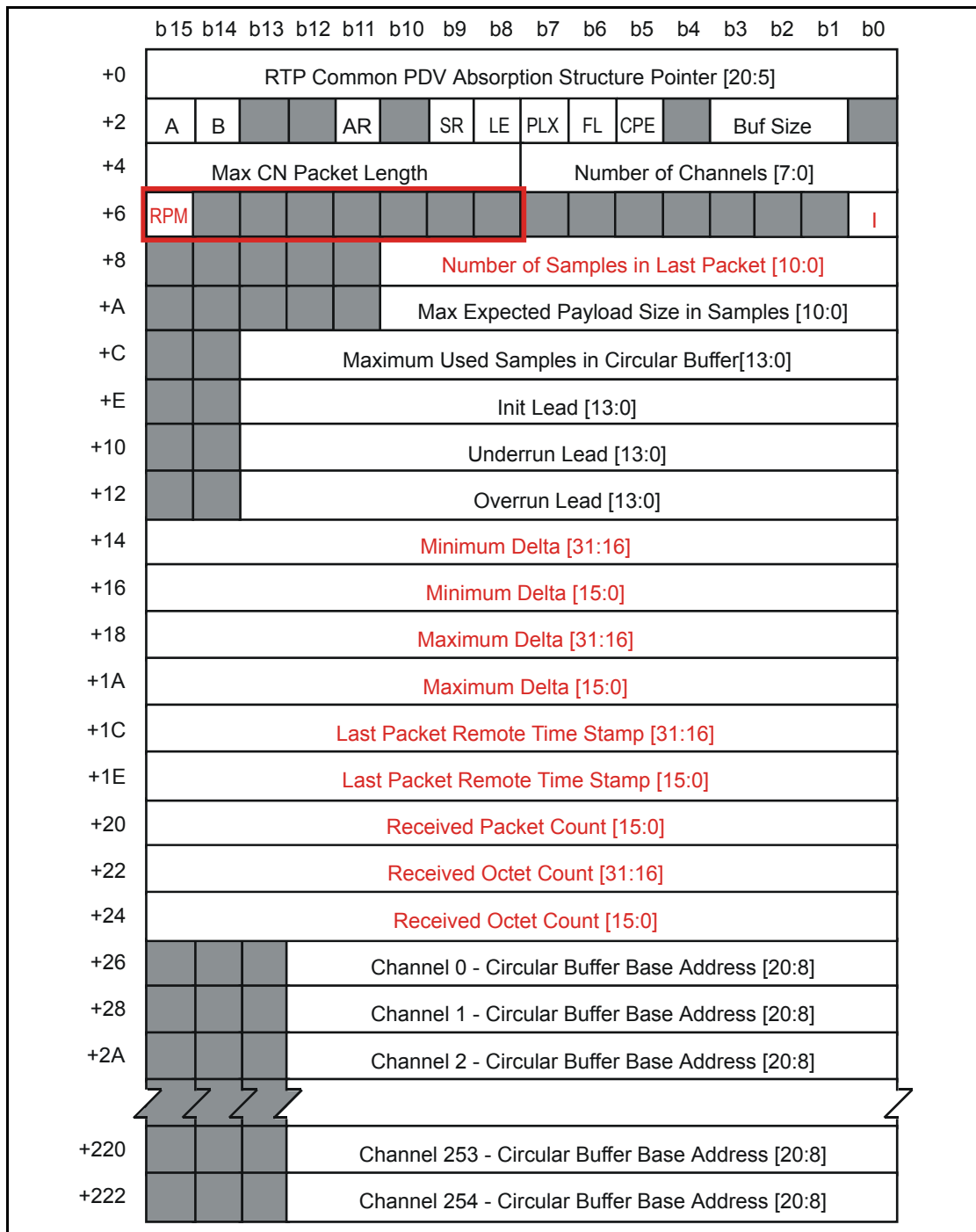
Figure 49 - RX RTP xxPCM Channel Structure
