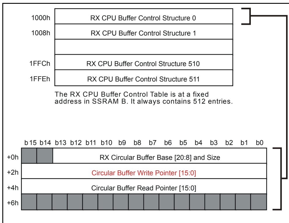
Figure 54 - Rx CPU Buffer Control Table
