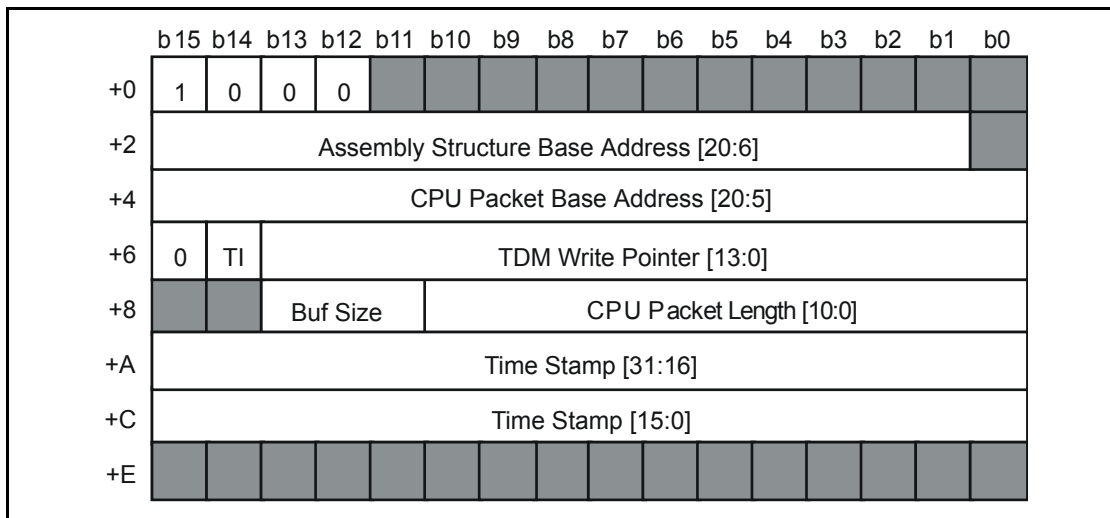
Figure 35 - Assembly Event - Send HDLC RTP Packet
