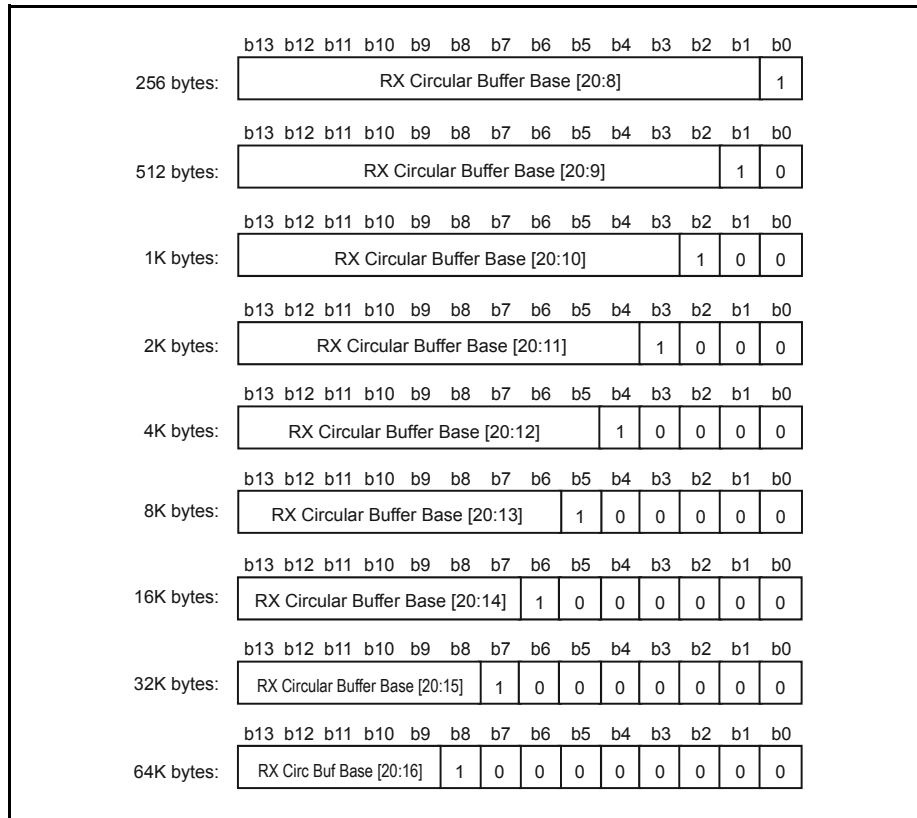
Figure 70 - RX Circular Buffer Base and Size
