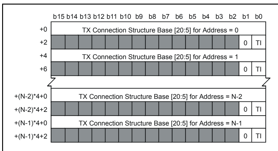
Figure 63 - HDLC Address LUT (RTP)
