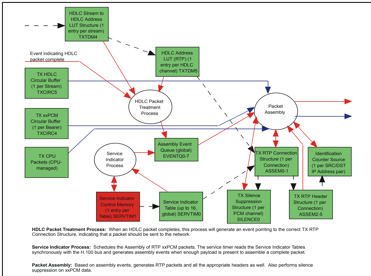
Figure 21 - Tx Flow 2
