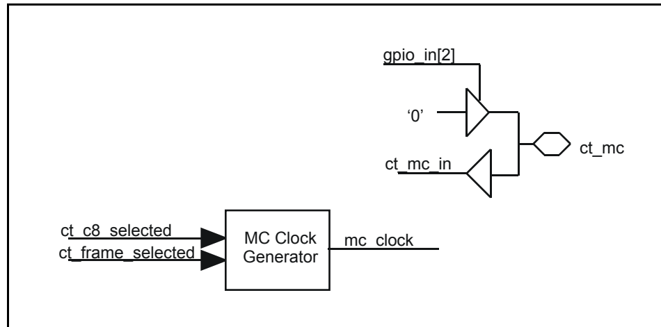
Figure 83 - Message Channel Circuit
