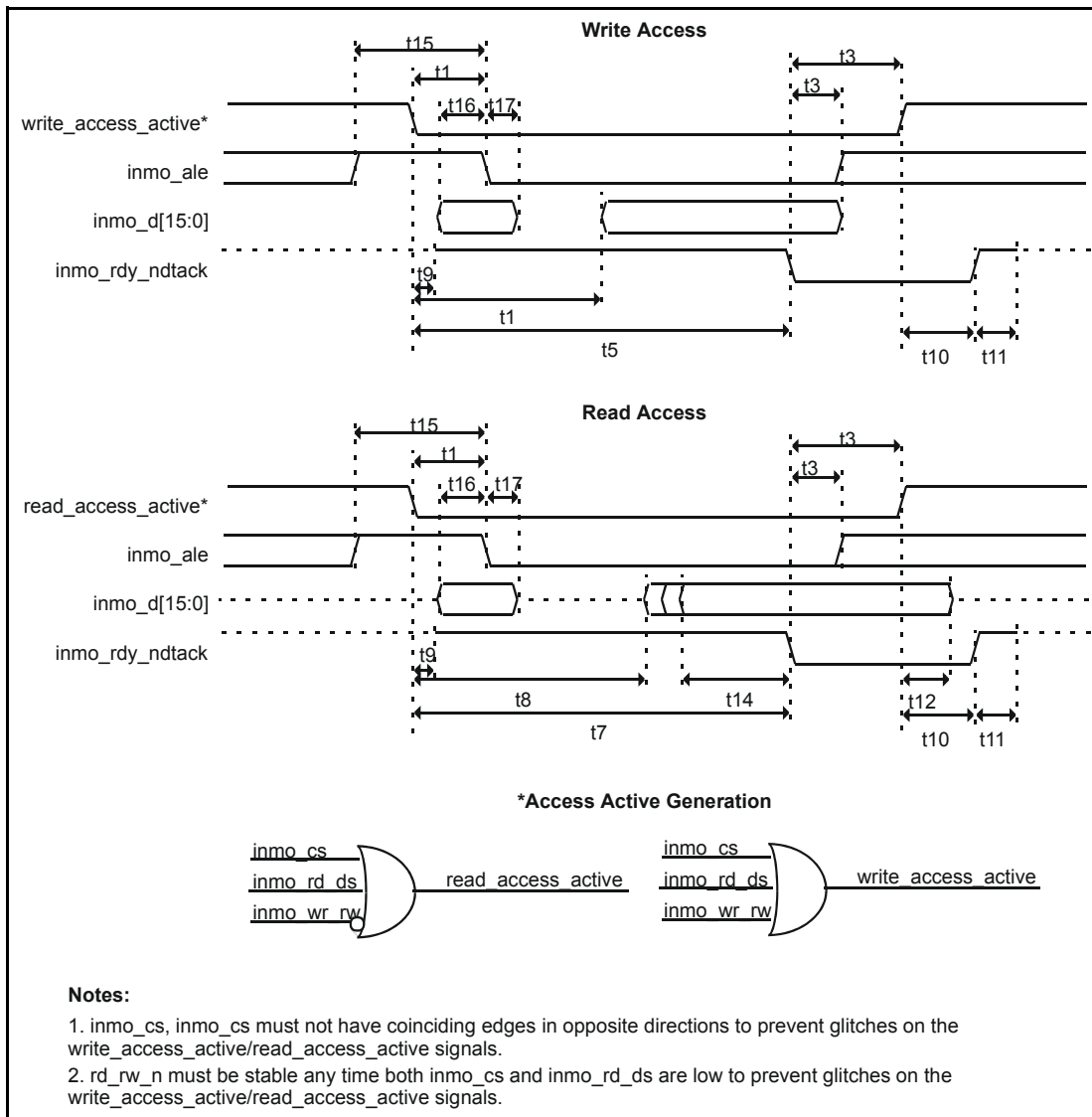
Figure 88 - Multiplexed CPU Interface - Motorola Mode
