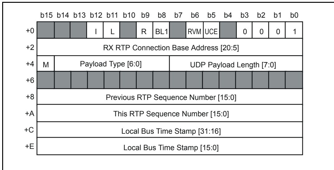
Figure 48 - RX Disassembly Event Report Queue - RTP Connection Report
