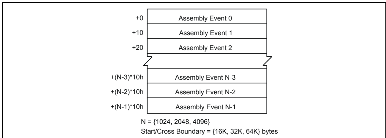
Figure 34 - Assembly Event Queue
