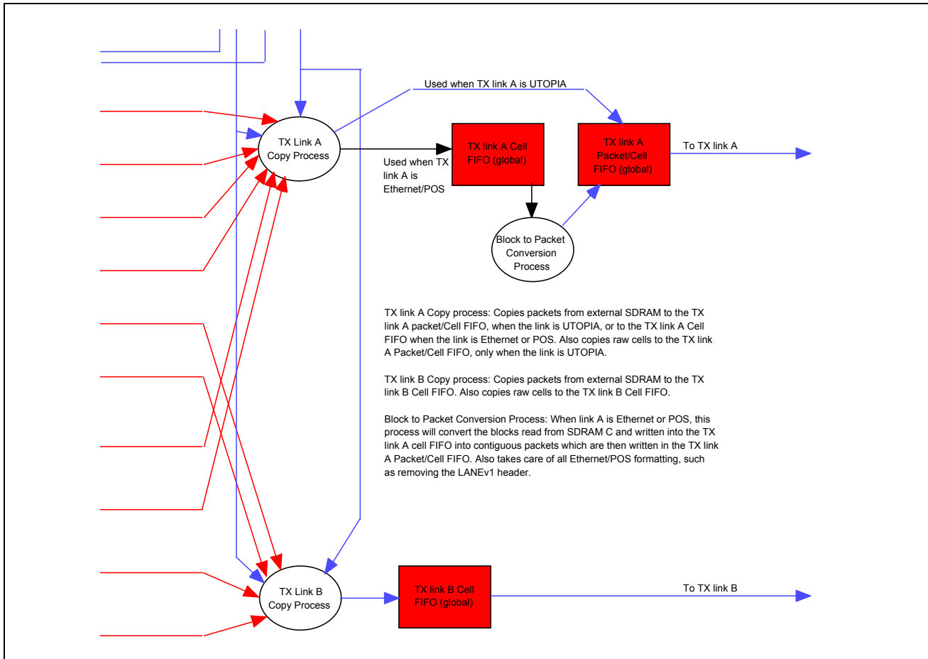
Figure 23 - Tx Flow 4
