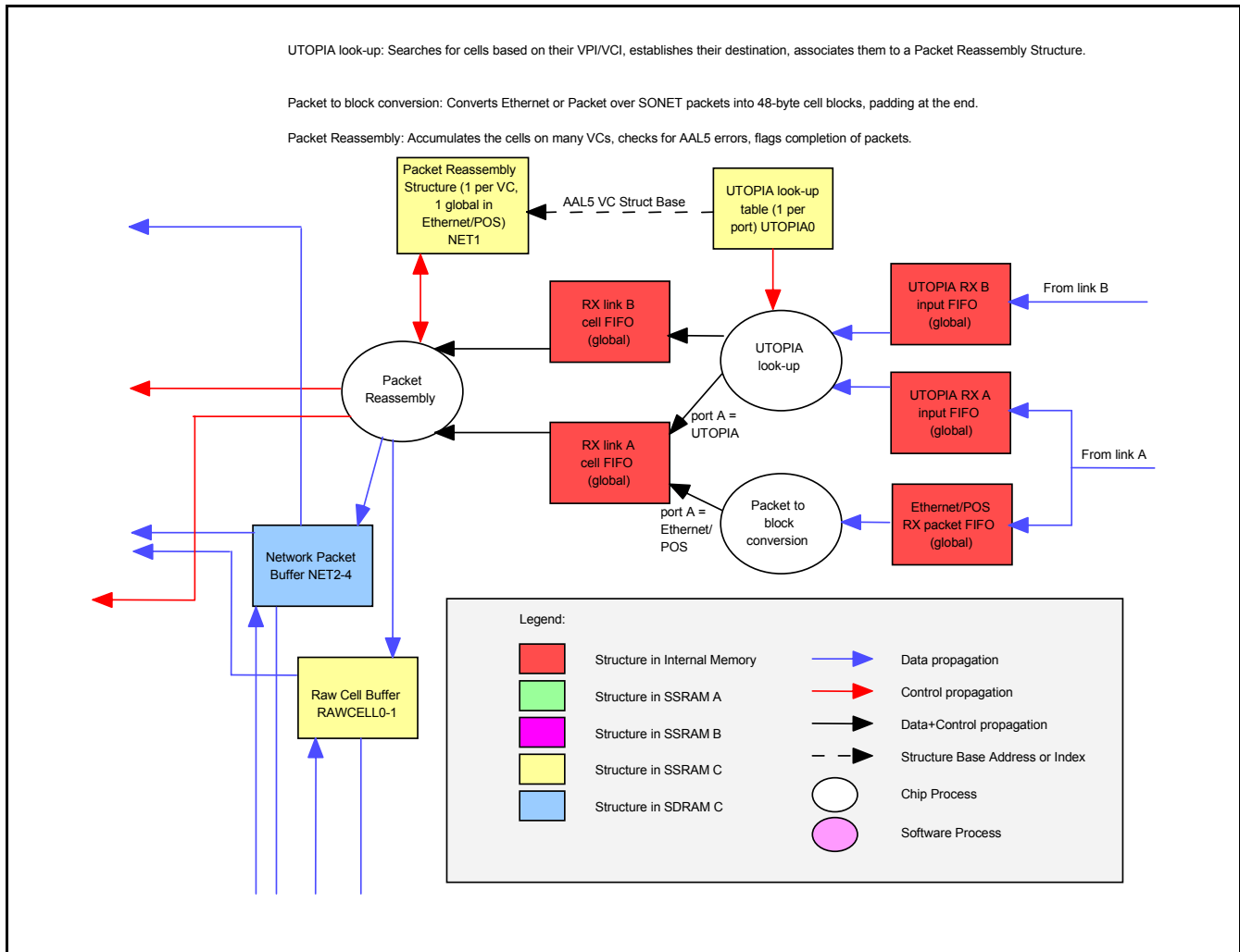
Figure 16 - Rx Flow 1
