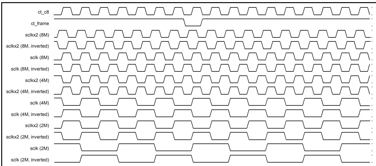
Figure 76 - TDM Bus Timing - sclkx2 Generation
