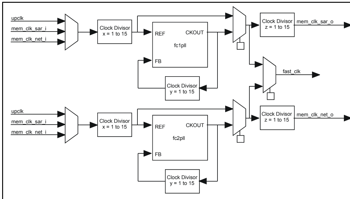
Figure 78 - Clock Synthesis
