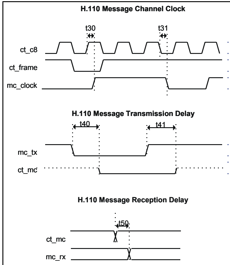
Figure 91 - H.110 Message Handling
