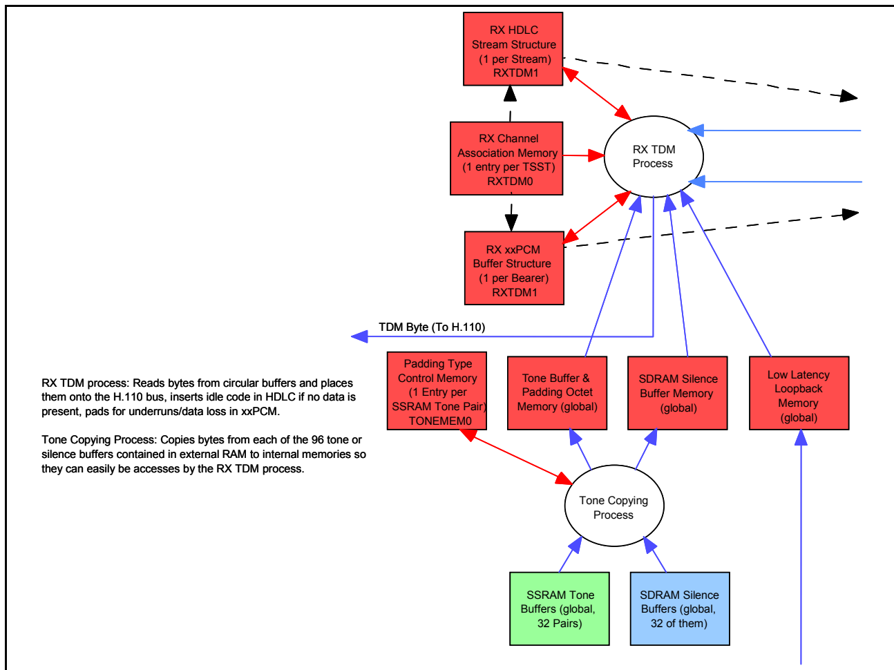
Figure 19 - Rx Flow 4
