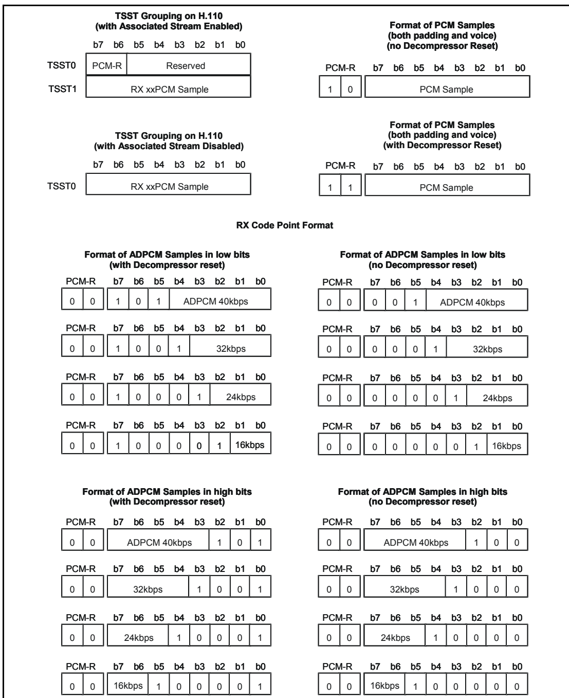
Figure 71 - Format of RX xxPCM TSSTs - 1 of 2
