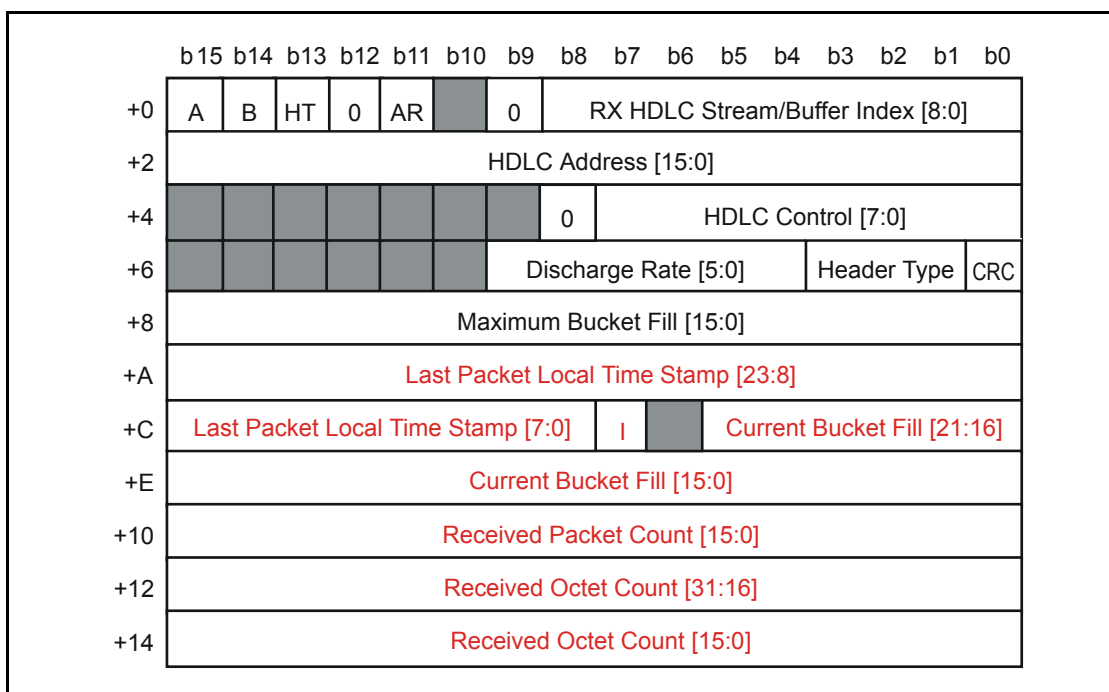
Figure 52 - RX RTP HDLC Channel Structure
