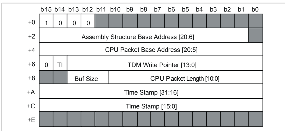
Figure 37 - Assembly Event - Send CPU RTP Packet
