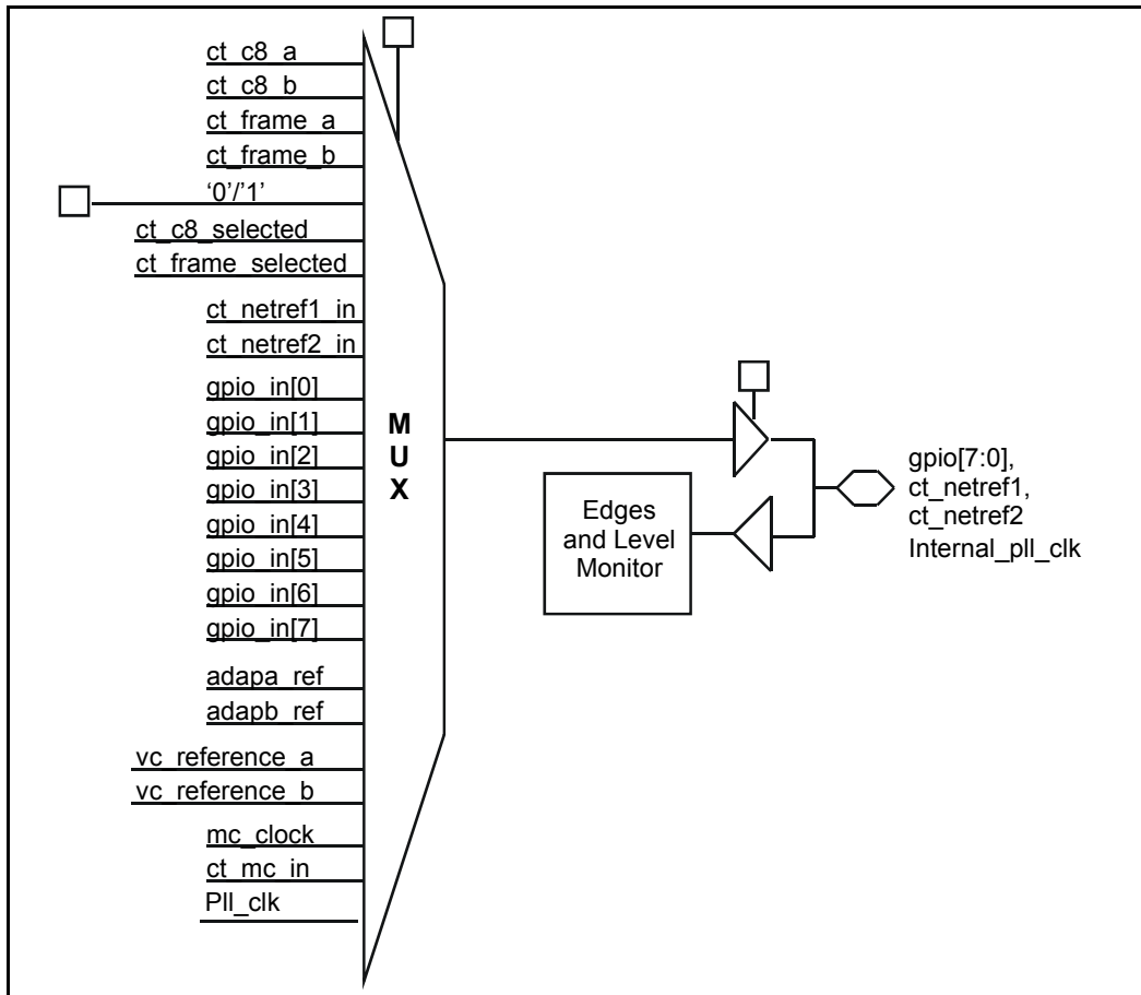
Figure 82 - GPIO Functionality
