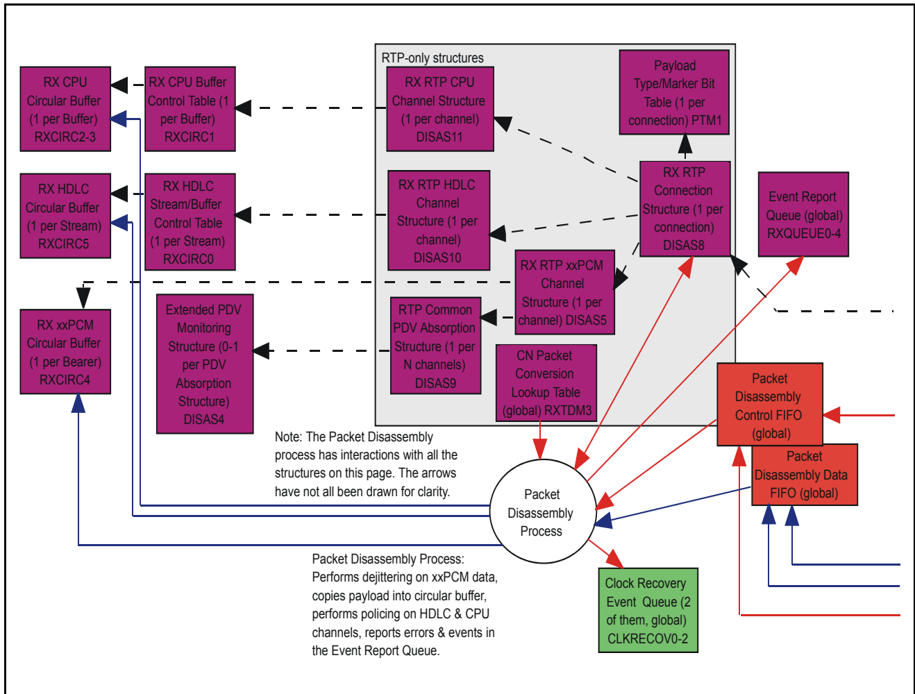
Figure 18 - Rx Flow 3
