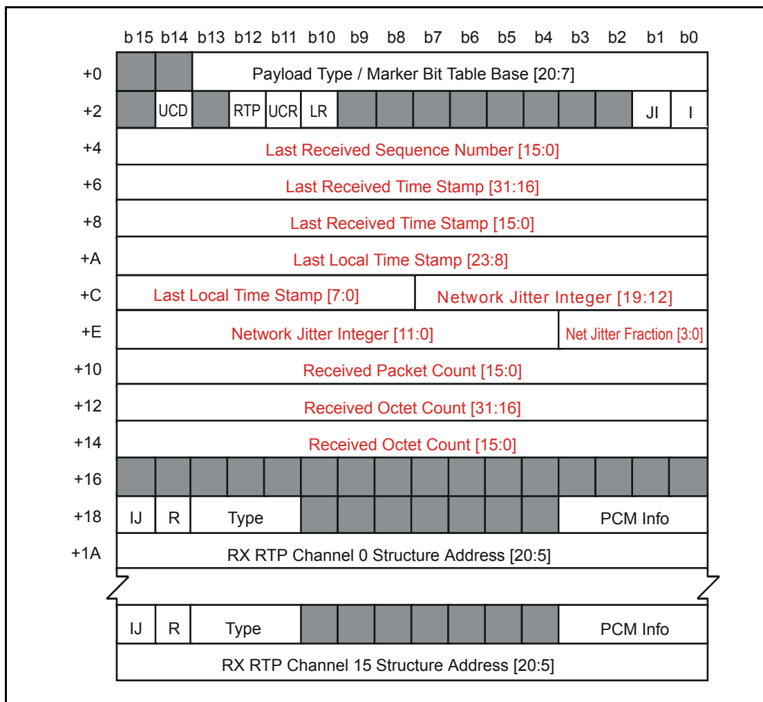
Figure 46 - RX RTP Connection Structure
