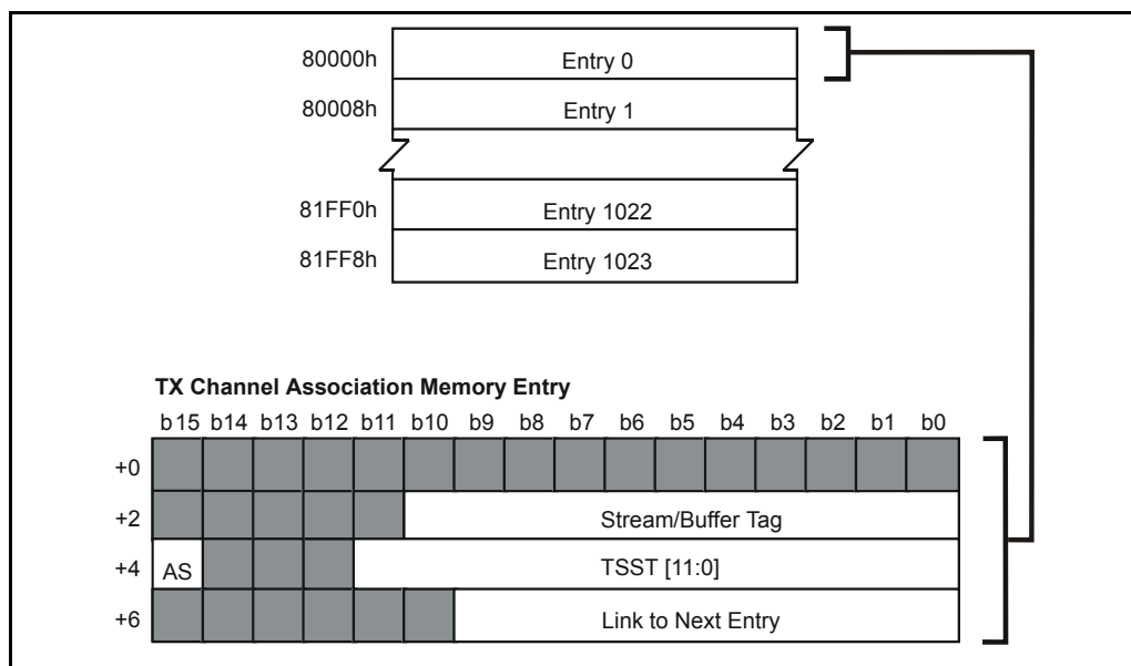
Figure 57 - TX Channel Association Memory
