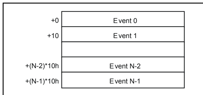
Figure 79 - Adaptive Clock Recovery Event Queue
