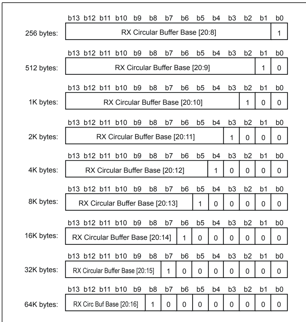
Figure 55 - RX Circular Buffer Base and Size
