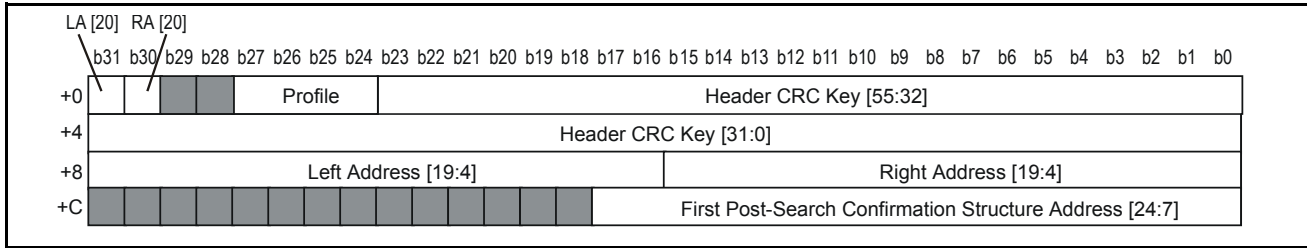
Figure 31 - Binary Tree Node
