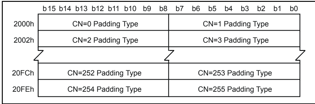
Figure 73 - CN Packet Conversion Lookup Table
