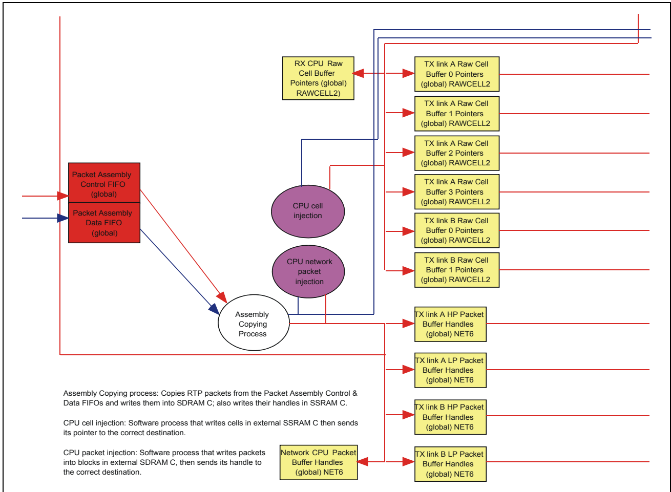
Figure 22 - Tx Flow 3
