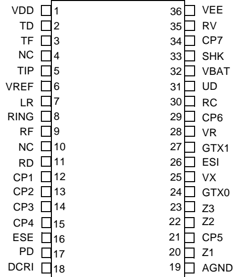
Figure 2 - Pin Connections
