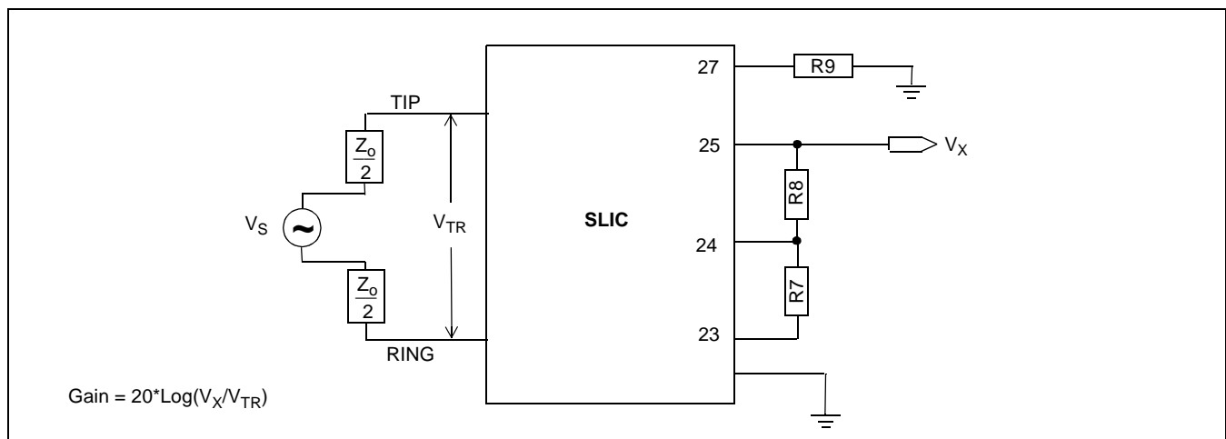
Figure 9 - 2-4 Wire Gain
