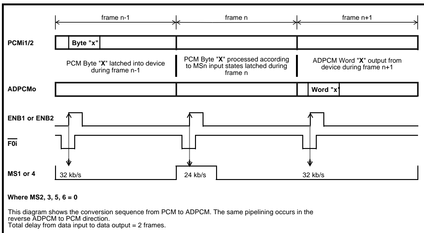
Figure 10 - Data Throughput
