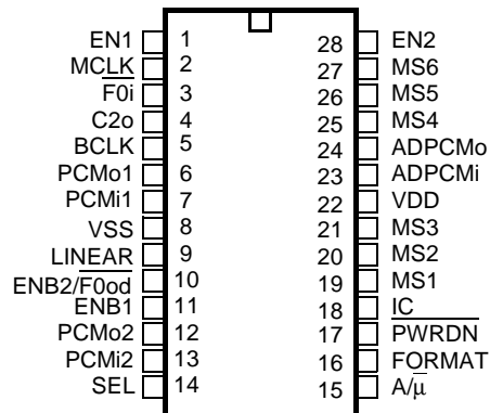
Figure 2 - Pin Connections
