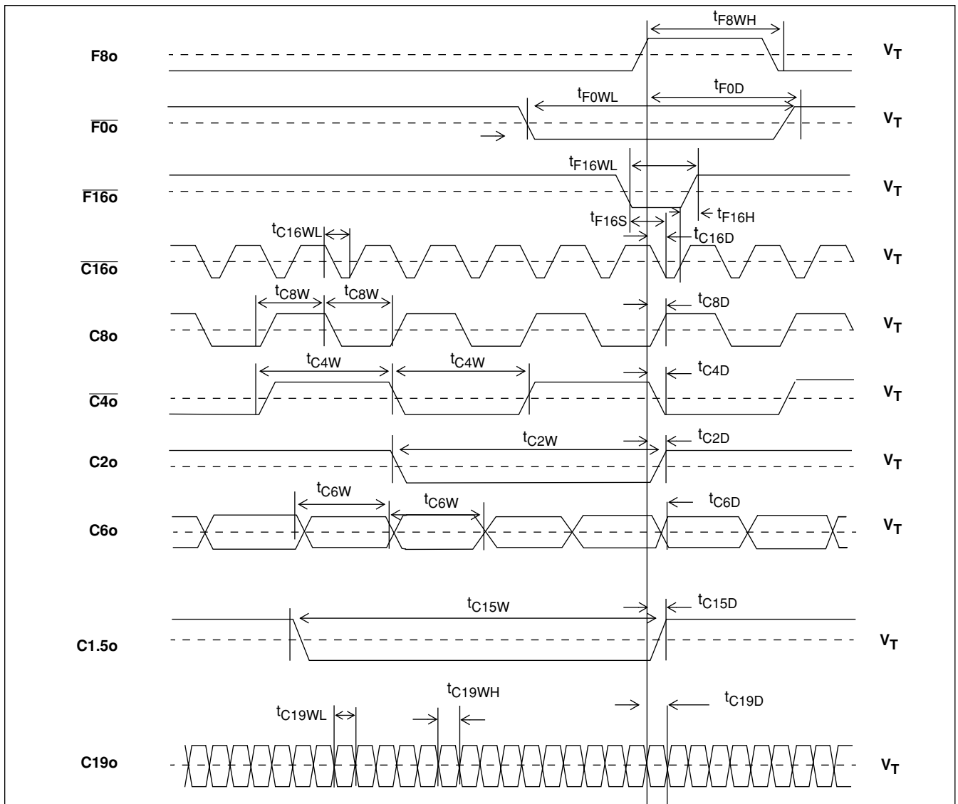
Figure 10 - Output Timing 1
