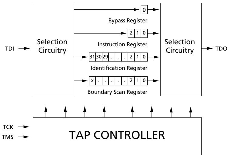
Figure 3 TAP Controller Block Diagram
