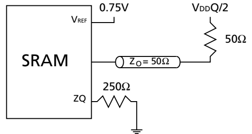
Figure 1 Output Load Equivalent
