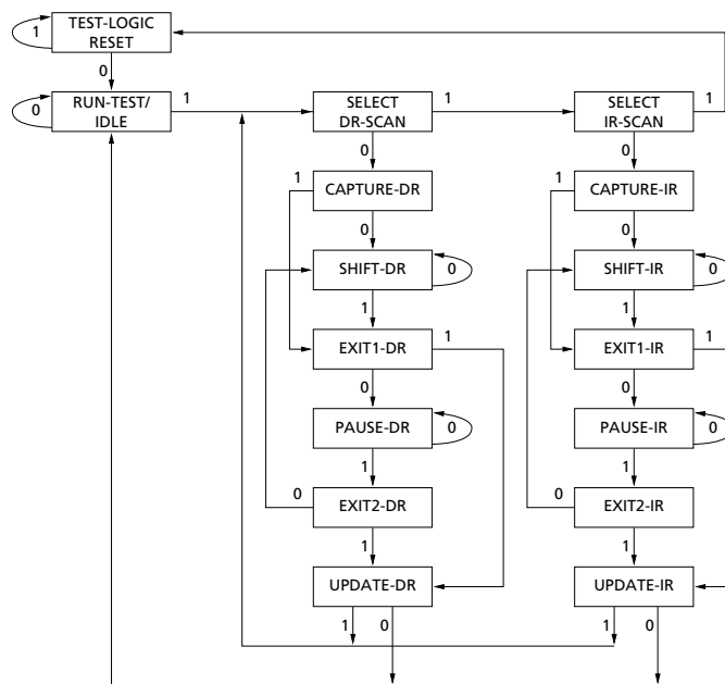
Figure 2 TAP Controller State Diagram
